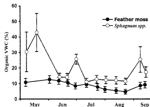
FIG. 1. Seasonal variation in VWC of shallow organic soils (10 cm below the ground surface) near Erickson Creek, Alaska (replotted from O'Donnell et al., 2009).
