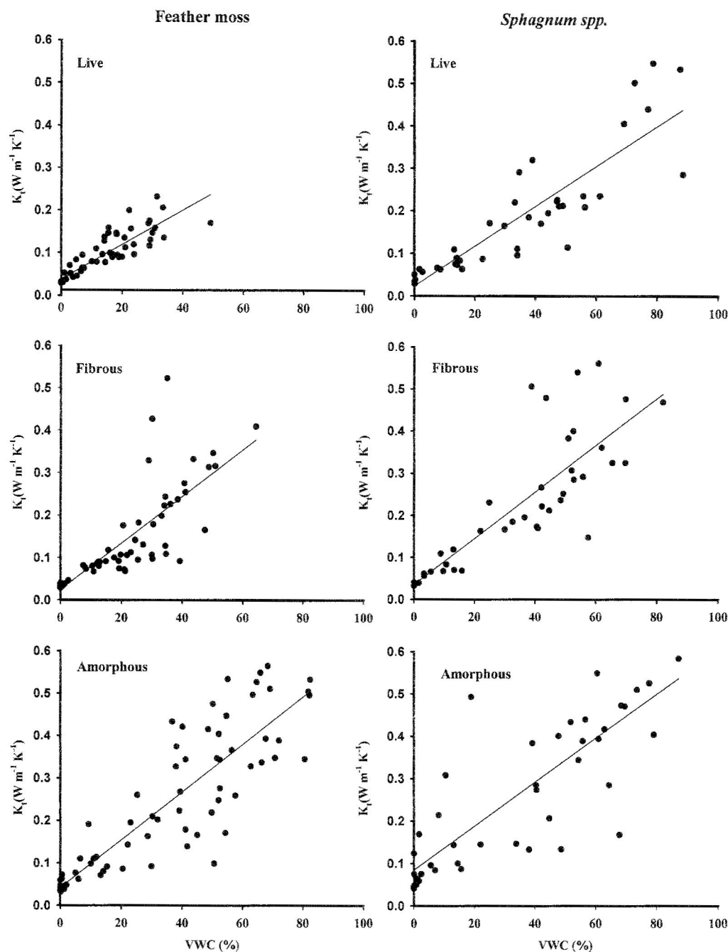
FIG. 2. The relationship between thawed thermal conductivity ( K_t ) and VWC within different moss and organic matter types. Regression techniques revealed a positive linear relationship between K_t and VWC for all samples types. Detailed regression statistics are reported in Table 2.
