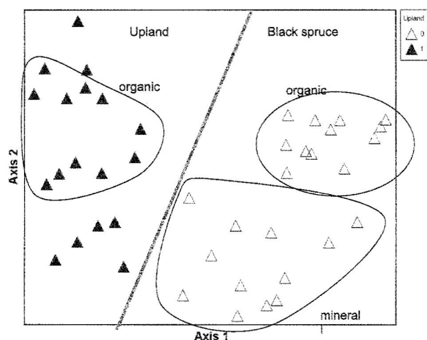
Fig. 3. NMS ordination of upland and black spruce ( Picea mariana ) sites with abundances across years combined. Note the strong split between upland and black spruce sites and further subdivision between organic and mineral communities. Upland sites are shown with solid triangles and black spruce sites are depicted with open triangles. Overlays have been manually added.
