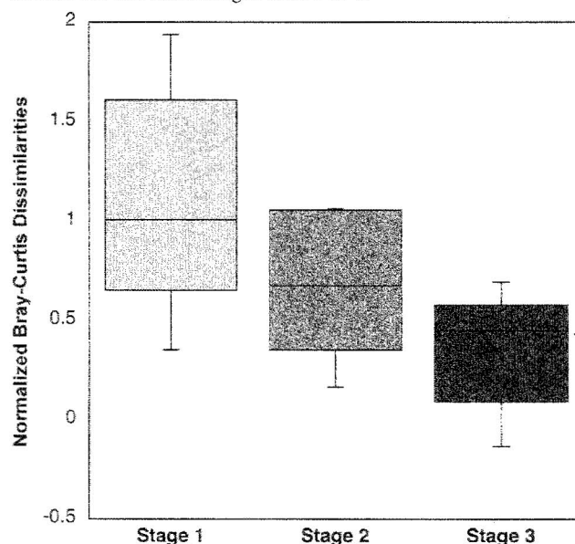
Fig. 5. Box plot of intersite Bray–Curtis dissimilarities by successional stage. Fungal abundances were normalized by site totals and the resulting pairwise Bray–Curtis dissimilarity values between replicate sites of a given successional stage were logit transformed because the raw index ranges from 0 to 1.
