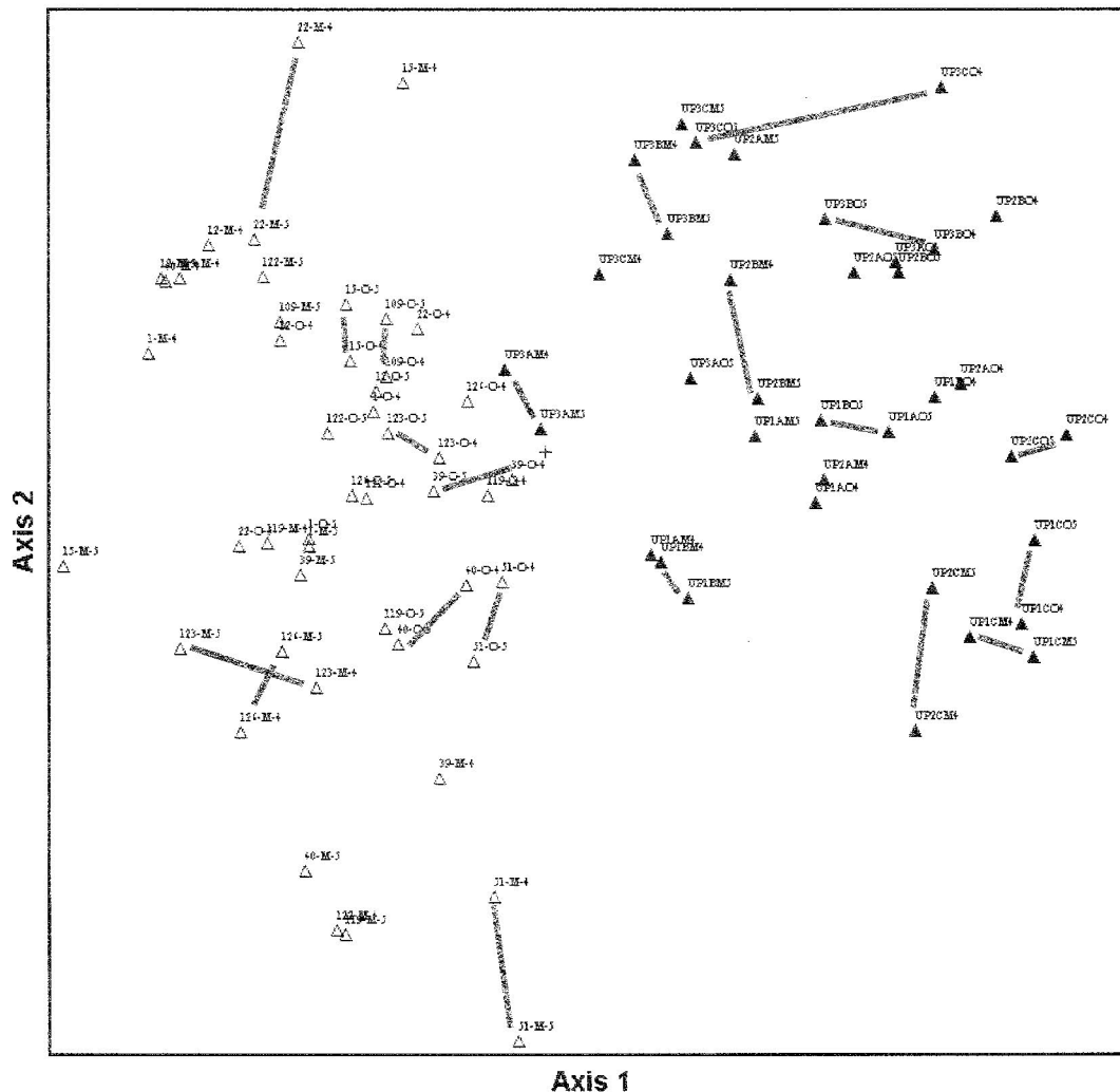
Fig. 2. NMS ordination of upland and black spruce ( Picea mariana ) sites. Lines connect samples from the same site and soil horizon in successive years (2004–2005), demonstrating the general consistency of communities at a site across years. For clarity, only a subset of year to year connections are shown. Upland sites are shown with solid triangles and black spruce sites are depicted with open triangles.
