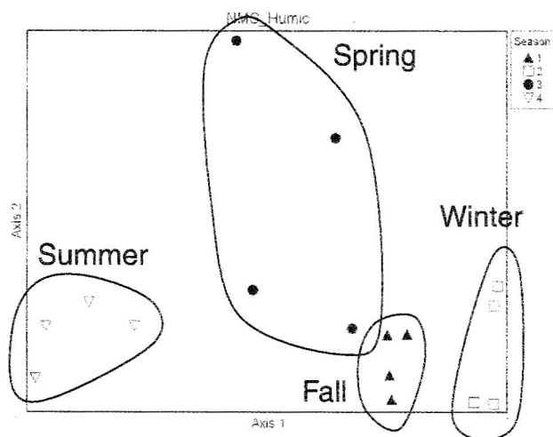
Fig. 6. NMS ordination plot from the seasonal study. The first two dimensions are plotted. Datapoints represent the communities of OTUs derived from the humic horizon across seasons and snow conditions.
