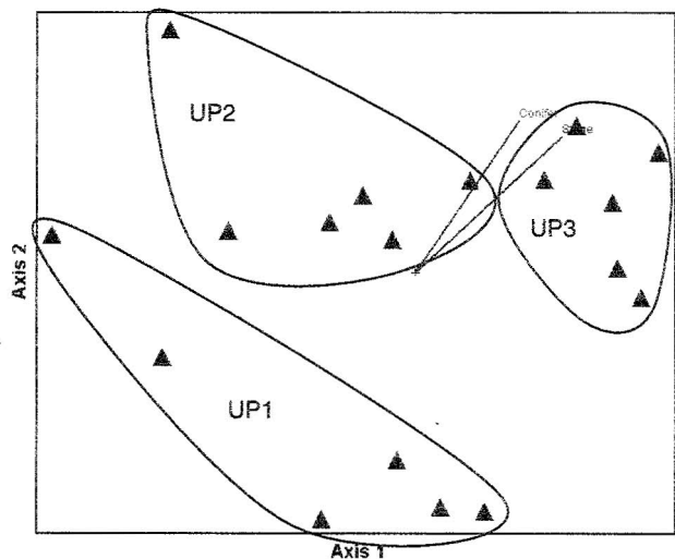
Fig. 4. NMS ordination of upland sites with years combined. Note strong clustering of replicate sites within each successional stage and greater intersite variation in the earliest UPI sites. Vectors are shown for environmental variables correlated with ordination axes at r^2 > 0.300 .
