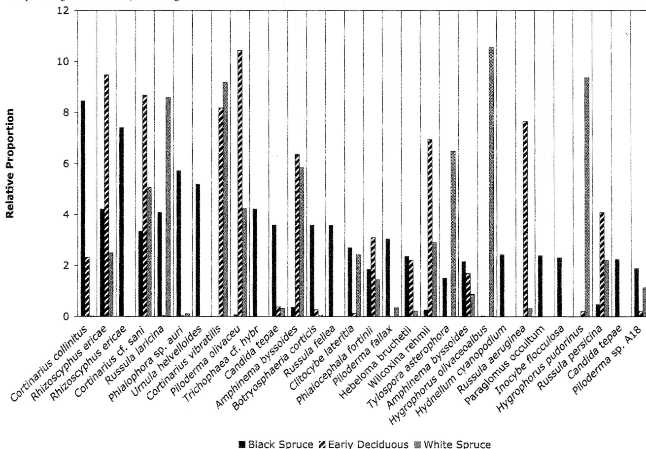
Fig. 1. Proportional rank abundances of the 30 most abundant OTUs by stand type. Early-successional deciduous sites are the upland UP1 and UP2 sites, white spruce ( Picea glauca ) are the upland UP3 sites, and the black spruce ( Picea mariana ) sites are mostly lowland. Numbers of clones for OTUs were normalized by the total numbers of clones recovered from each stand type. The OTUs are named by the top identified BLAST hit in GenBank; note that some of the OTU sequences are rather divergent from their best match in GenBank and so likely belong to different species or genera than those listed.
