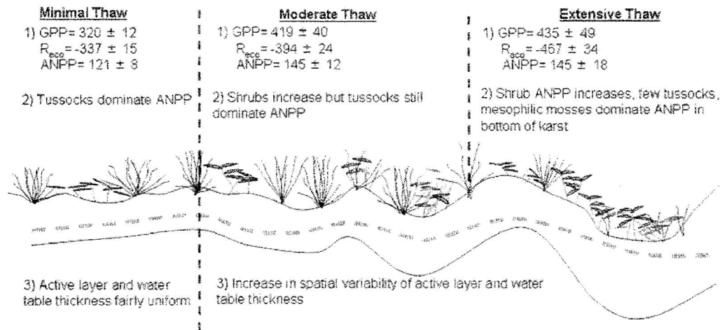
Figure 8. Summary of gross primary productivity (GPP, \text{g CO}_2\text{-C m}^{-2} \text{ yr}^{-1} ), ecosystem respiration ( R_{eco} , \text{g CO}_2\text{-C m}^{-2} \text{ yr}^{-1} ), and aboveground net primary productivity (ANPP, \text{g C m}^{-2} \text{ yr}^{-1} ) and conceptual diagram linking these fluxes to the changes in vegetation dominance of ANPP, active layer thickness (solid line), and water table height (dashed line) with increasing occurrence of thermokarst. Note that the depth to water table is similar at the site level, but within the Extensive Thaw site, water tends to pool where the active layer thickness is the greatest.
