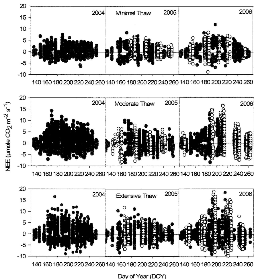
Figure 2. All net ecosystem exchange (NEE) and ecosystem respiration ( R_{eco} ) data collected during the growing season. Open circles are automated chamber (2005 and 2006), and closed symbols are manual chamber measurements. Negative values are C loss from the ecosystem.
