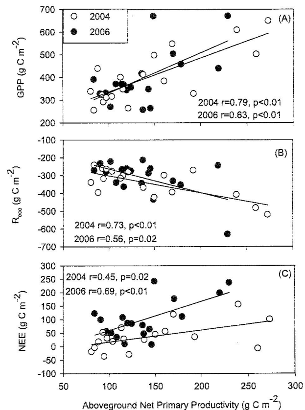
Figure 7. Relationship between aboveground net primary productivity (ANPP) and growing season (May–September) \text{CO}_2 -C exchange for 2004 and 2006. ANPP was not measured in 2005.
