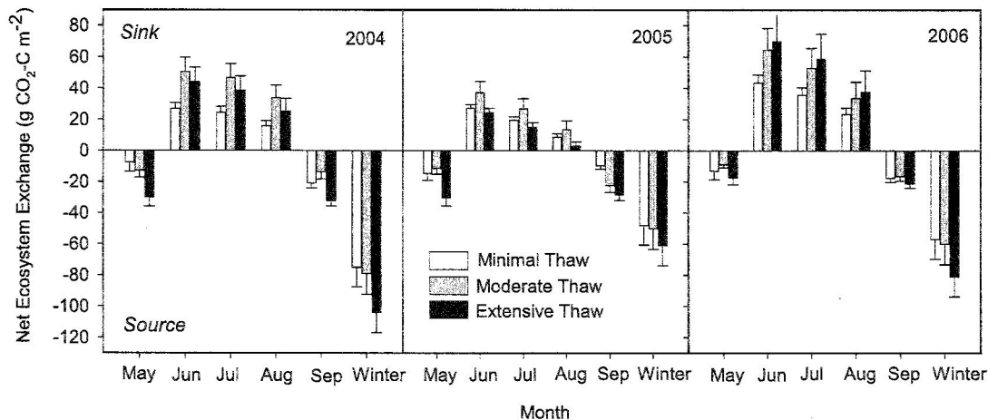
Figure 4. Modeled monthly NEE and winter R_{eco} (average \pm stderr) for three sites varying in degree of permafrost thaw over 3 years of measurement.
