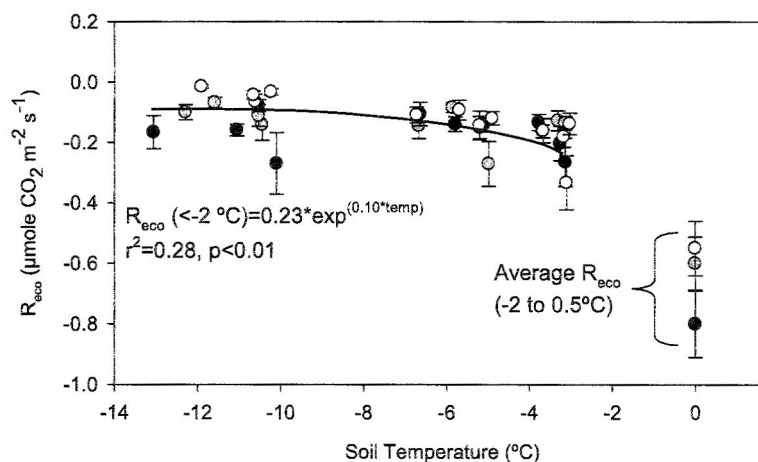
Figure 3. Response of ecosystem respiration ( R_{eco} ) during winter to integrated soil temperature averaged across 10, 20, 30, and 40 cm depths. Winter R_{eco} values measured between -2 and 0.5^\circ\text{C} were not significantly related to temperature, but increased dramatically relative to respiration at colder ( <2^\circ\text{C} ) temperatures. Below <2^\circ\text{C} , R_{eco} and temperature were significantly correlated but the exponential relationships were not significantly different across sites.
