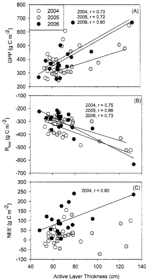
Figure 6. Relationship between active layer thickness and growing season (May–September) \text{CO}_2 -C exchange. All data with an associated linear fit line and a correlation coefficient ( r ) have a p value that is <0.01 .
