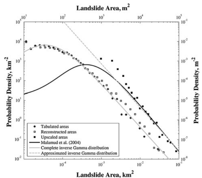
Fig. 3 Probability density of the landslide areas for the tabulated, reconstructed and upscaled data. The inverse gamma distribution obtained by Malamud et al. (2004) ( black line ), and the complete and approximated inverse gamma distribution fitted to the data from this work ( continuous and dashed grey lines )
