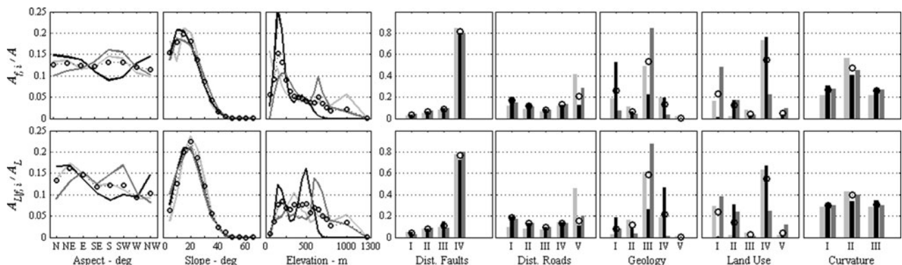
Fig. 4 NOLS ( A_f/A ) and LS ( A_{L|f}/A_L ) area distributions for all eight inducing factors: light grey lines and bars for Blanco basin, black for Cibuco basin, and dark grey for Coamo basin. The circles are for the case when all the three basins are considered together
