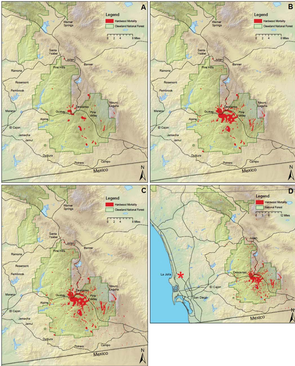
Fig. 1. Distribution of oak mortality (red areas) caused by the goldspotted oak borer, Agrilus auroguttatus , in San Diego Co., California. A) 2002 to 2004, B) 2002 to 2007, C) 2002 to 2010. This area ranges from 32°42'09.90"N, 116°20'34.67"W to 32°49'41.60"N, 116°51'30.33"W to 32°36'31.45"N, 116°28'06.77"W to 33°11'58.64"N, 116°42'37.96"W. Location of satellite infestation (southwest of red * in map D) found in 2009 is Marion Bear Memorial Park near La Jolla.
