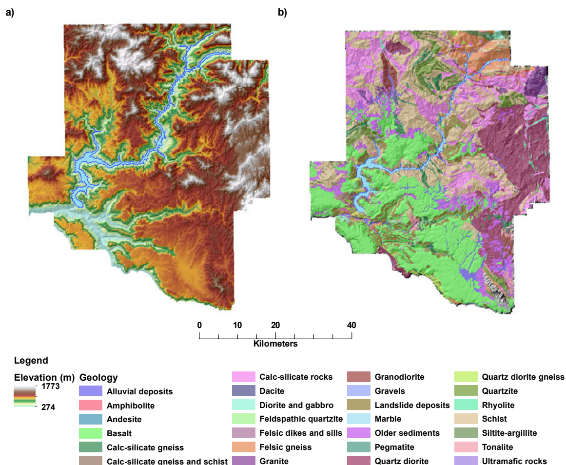
Figure 2. (a) Elevation gradients across the northern Idaho ID612 survey area within the Northern Rockies ecoregion, USA [34]. The blue water body represents the outline of Dworshack Reservoir on the North Fork of the Clearwater River. (b) Geologic parent material across the ID612 survey area representing extrusive and intrusive igneous rocks, metasedimentary and metamorphic rocks, with minor components of unconsolidated deposits [34].
