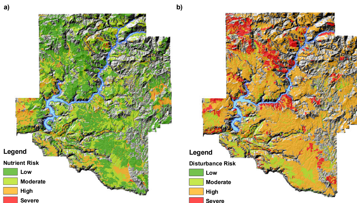
Figure 5. (a) Nutrient risk assessment to long-term soil productivity following ground-based harvest activities in the ID612 survey area of the Northern Rockies ecoregion, USA; (b) Soil disturbance risk assessment to long-term soil productivity following ground-based harvest activities in the ID612 survey area. Gray scale areas represent excluded landforms with >45 percent slope [35].
