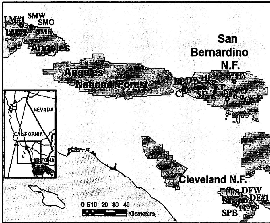
Fig.1. Map of study area with sites from 2008 surveys. Site codes are defined in Table 1.
