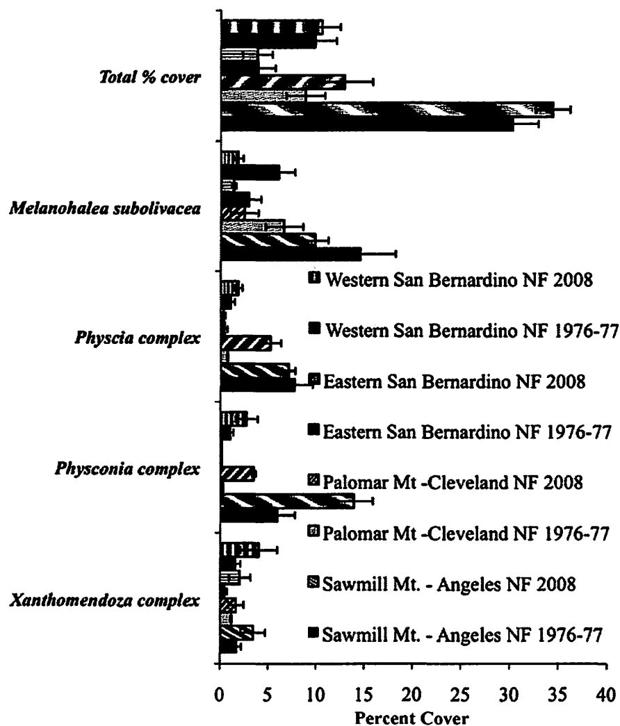
Fig. 3. Comparison of percent cover of four taxa from Sigal (1979) with percent cover from 2008 surveys on Quercus kelloggii bark. Error bars represent one standard error from the mean. See Table 2 for definitions of the species complexes.
