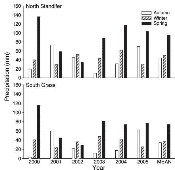
Fig. 2 Mean seasonal precipitation totals and yearly seasonal totals for rain gauges near the North Standifer sagebrush study site and the South Grass shadscale study site for each year (August through May) over the 6-year period of the study. Autumn precipitation includes August through November, winter precipitation includes December and January and spring precipitation includes February through May.
