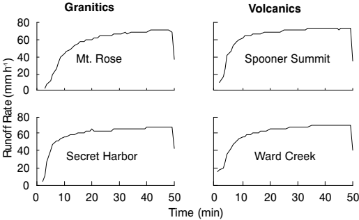
Figure 2. Composite hydrographs ( n = 6 ) during rainfall simulations at four Lake Tahoe locations. Rainfall rates were 86 mm h -1 .
