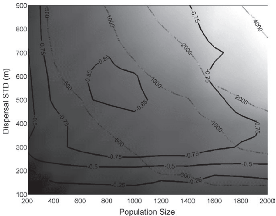
Fig. 20.5 Correlation length of habitat occupied by a minimum of five individuals per hectare for the Roads scenario. The dashed contours indicate correlation length of dispersal habitat. The solid contours indicate the proportional decrease in correlation length in the Roads scenario from that of the Null scenario. Over 60% of the life-history space is predicted to experience at least a 75% reduction of occupied habitat correlation length due to roads in comparison with the null scenario, and approximately 10% of the life-history space experiences over 85% reduction in habitat connectivity
