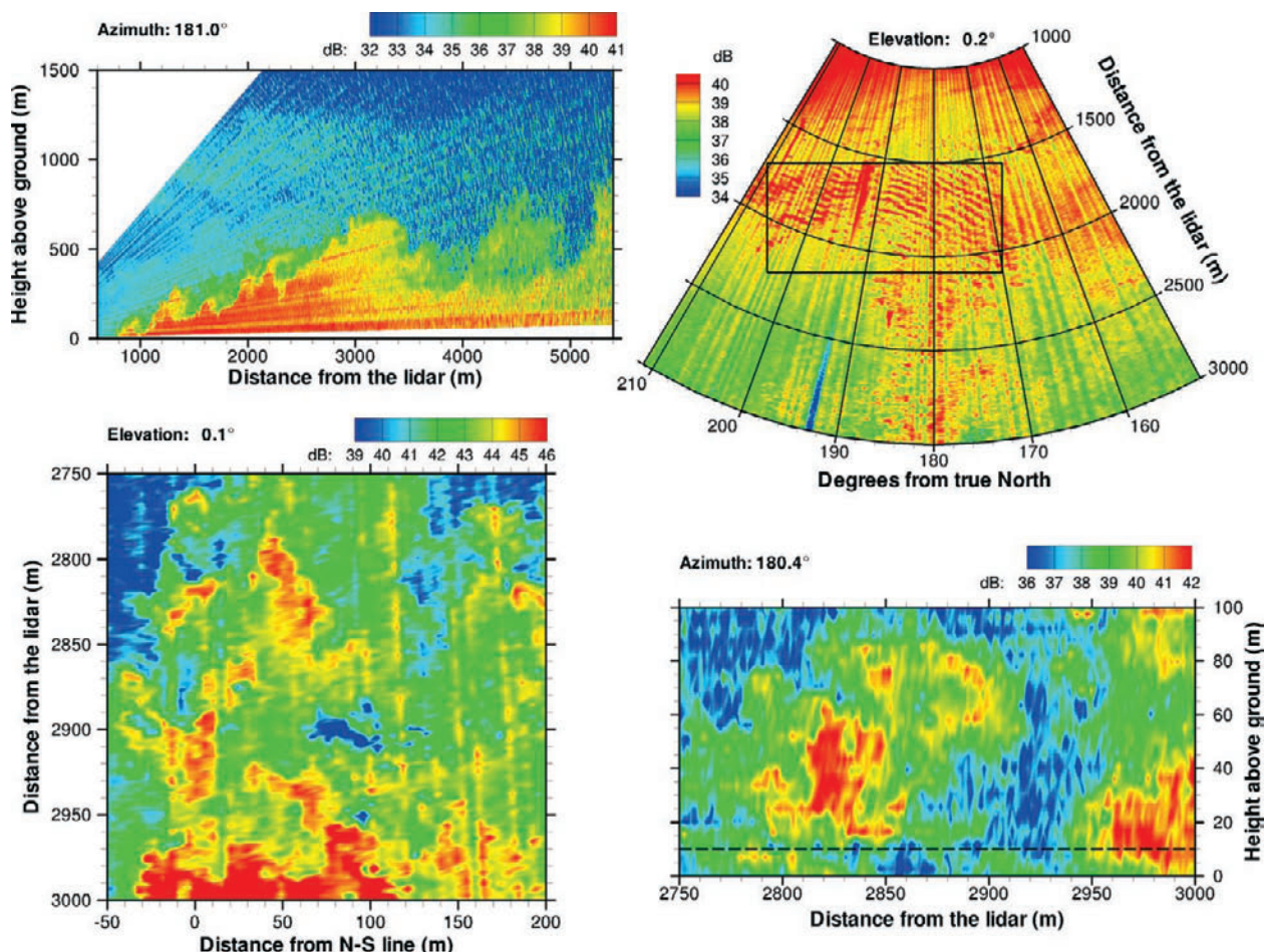
FIG. 13. Four images of aerosol backscatter intensity (dB) from REAL during CHATS. (top left) An RHI scan at 0111 UTC 1 May (1811 LT Apr 30) at azimuth 181° (or nearly due south) depicting the passage of a sea-breeze front traveling from right to left; note the evolving length scales (from left to right) participating in the entrainment process between the two different density fluids. (top right) A PPI scan at an elevation 0.2° above the horizontal taken at 1349 UTC 25 Apr (0649 LT 25 Apr) showing canopy-scale gravity waves induced by velocity shear and thermal stratification at the canopy top; Cilker Orchards is roughly contained within the rectangle. (bottom left) A near-horizontal PPI scan (elevation 0.1° above the horizontal). (bottom right) An RHI scan (azimuth 180.4° or nearly due south). These lower two panels focus in on the near-canopy region and therefore only depict a fraction of the total region scanned by REAL. The horizontal slice (bottom left) is from 2353 UTC 24 May (1653 LT 24 May), and the vertical slice (bottom right) is from 2344 UTC 24 May (1644 LT 24 May). The dashed line (bottom right) depicts the top of the canopy. Note that REAL was able to sample RHI slices down into canopy because of orchard pruning and that its high resolution permits sampling of canopy-scale motions as well as the full PBL-scale flow.
