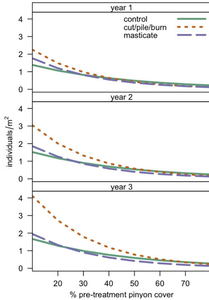
Figure 5. Shrub density.
