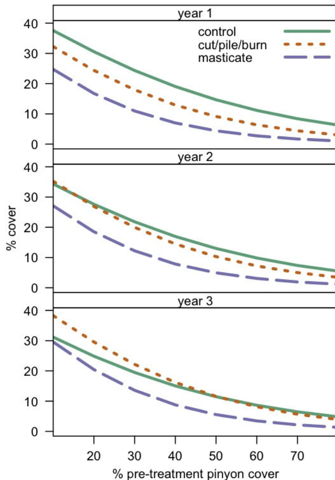
Figure 4. Shrub cover.
