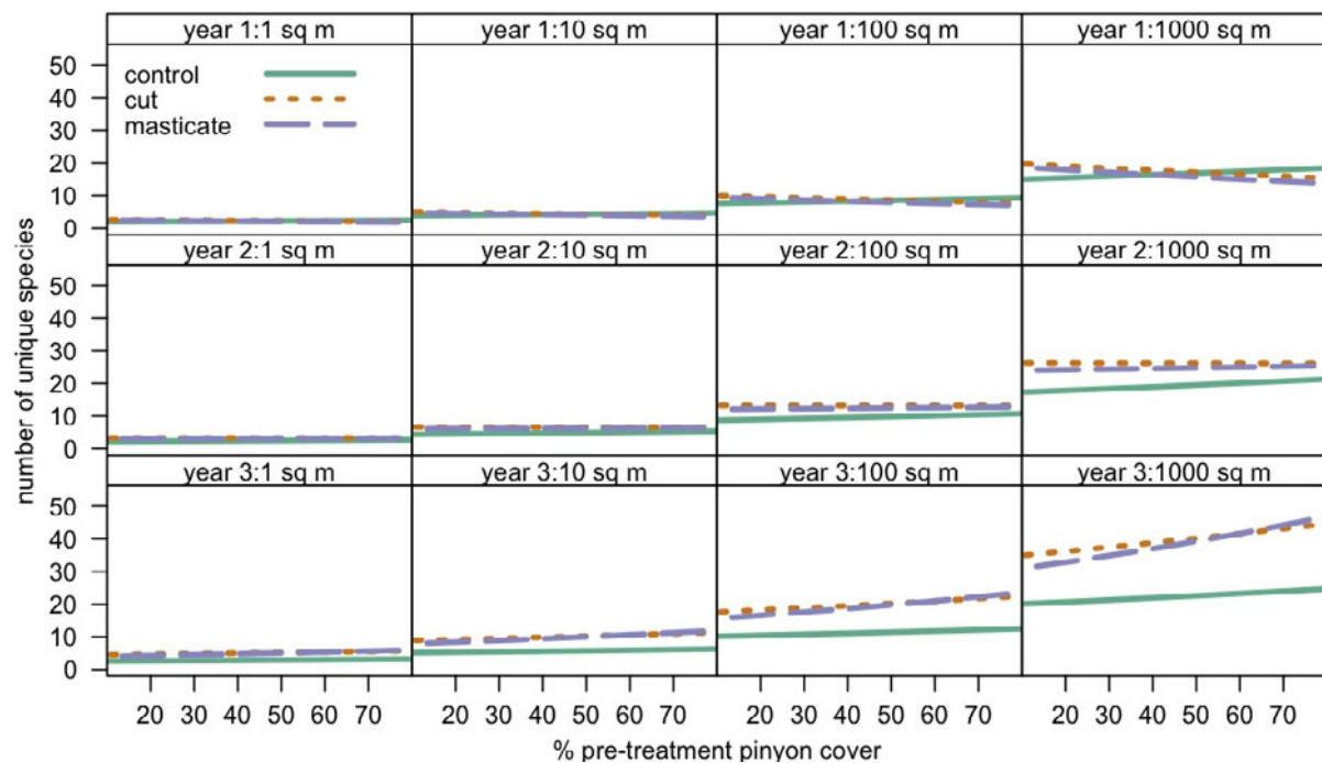
Figure 10. Species richness.
