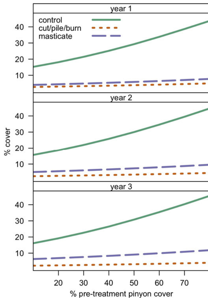
Figure 3. Tree cover.
