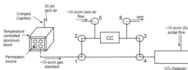
Fig. 1. A schematic diagram of the TOC calibration system. Gas standards are selectively passed over a palladium catalyst (CC). The \text{CO}_2 generated via oxidation of a standard is then measured using NDIR. During a background measurement, valves 1 and 4 open to allow flow to bypass the catalyst. At this time, valves 2 and 3 are closed shut and valves 5 and 6 are opened to flush the catalyst with zero air. To make a total carbon measurement, valves 2 and 3 opened, 5 and 6 closed, and valves 1 and 4 are switched to allow the sample to flow through the catalyst with the outflow to the \text{CO}_2 detector.
