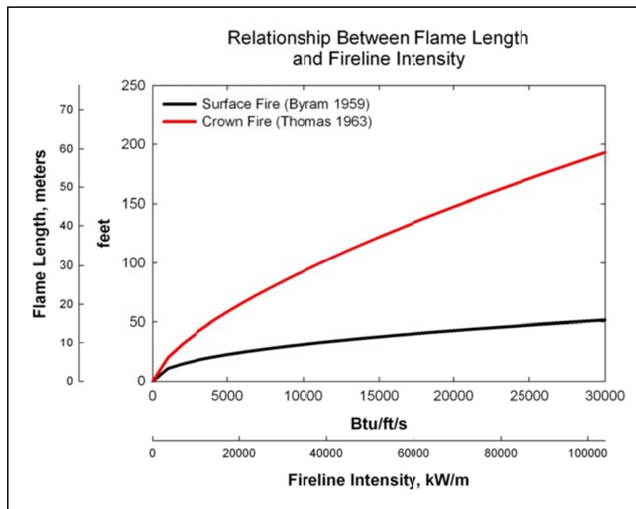
Fig. 6. Differences between Byram's and Thomas' flame length models are apparent as fireline intensity increases.
