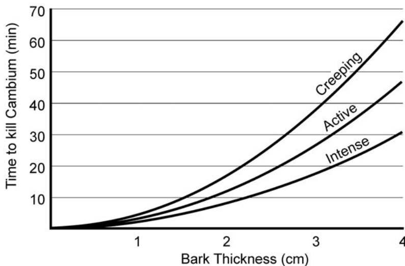
Fig. 6. The time to kill cambial tissue varies with the square of bark thickness and the difference between the stem's initial temperature (~ambient) and the stem's surface temperature due to radiant and convective heat transport from the flames. Stem surface temperature varies somewhat with the emissivity of the flames. Emissivity in turn increases with the flame depth as fire intensity increases until it approaches unity at around 1 meter flame depth. (from Ryan 1998, Cochrane and Ryan 2009)
