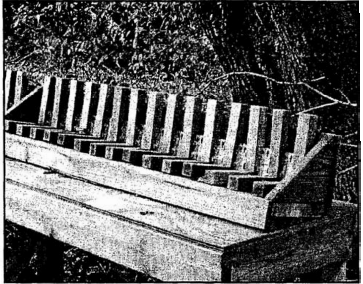
Figure 4. L-joint specimens are configured to trap moisture with the intent of accelerating fungal colonization.
