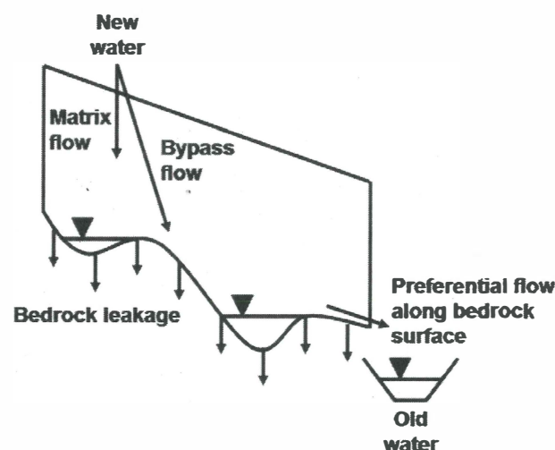
Fig. 11. New perceptual model of lateral subsurface flow at the Maimai hillslope.
