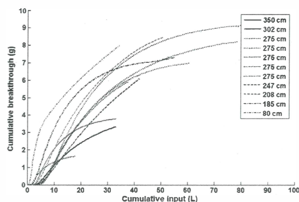
Fig. 9. Cumulative tracer breakthrough from surface applications, with 0.8–3.5 m soil remaining between tracer application and exposed soil face. 15 g of tracer was added for each application.
