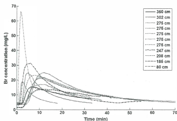
Fig. 7. Tracer breakthrough at trench face of Br-tracer applied on soil surface. Tracer was applied 4 m upslope of the trench, with 0.8–3.5 m soil remaining between tracer application and exposed soil face.
