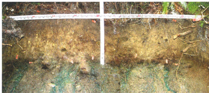
Fig. 5. Exposed evidence for preferential flow at the soil bedrock interface. (a) Preferential flow during experiment at soil bedrock interface with live roots. (b) Organic staining on bedrock surface indicating persistent flow at the soil bedrock interface.
