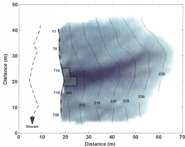
Fig. 2. Maimai instrumented hillslope with excavation locations (grey box). Selected trench sections (T1–T20) are labeled.
