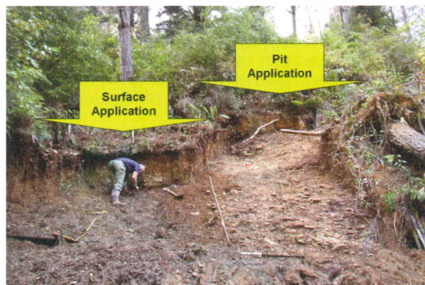
Fig. 4. Exposed bedrock surface with locations of surface and soil bedrock interface water and tracer applications.
