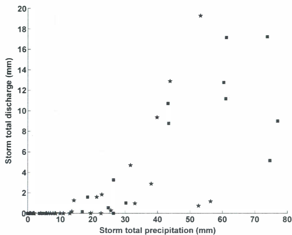
Fig. 1. Whole storm precipitation and hillslope discharge at instrumented Maimai hillslope. 150 days of monitoring included 125 storms (data from Woods and Rowe (1996) (stars) and Brammer (1996) (squares)).
