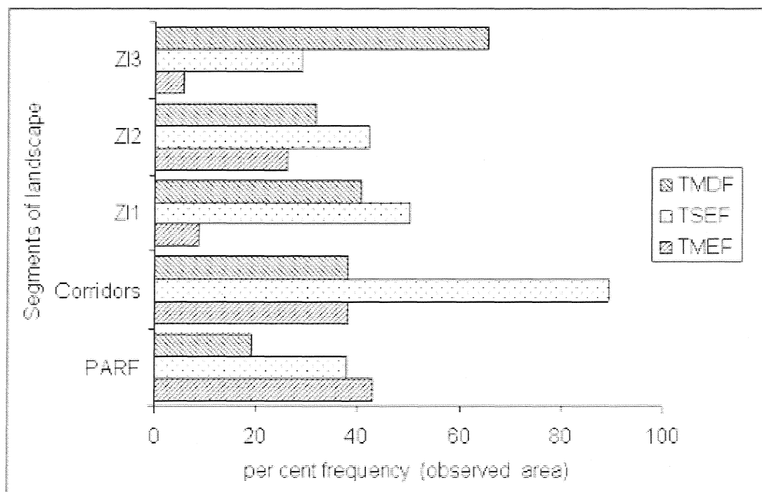
Fig. 5 Observed per cent area of various forest types among various landscape segments. TMEF = Tropical Evergreen Forests, TSEF = Tropical Semi-evergreen Forests, TMDF = Tropical Moist Deciduous Forests
