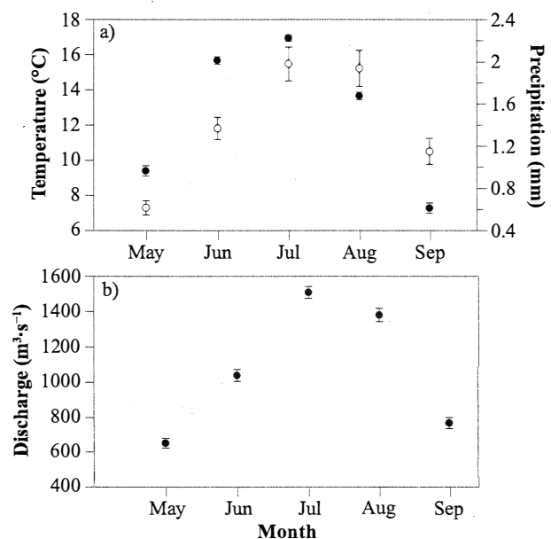
FIGURE 1. Temporal variation (May–September) in (a) air temperature (solid circles) and precipitation (open circles) in Fairbanks, Alaska (1930–2008) and in (b) Tanana River discharge in Nenana, Alaska (1962–2009). Data are monthly means \pm SE.
