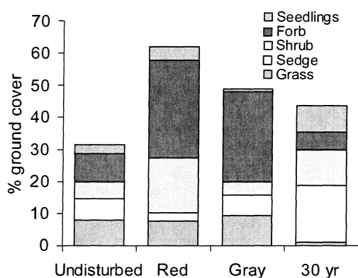
Fig. 2. Understory cover by plant functional group across a chronosequence of mountain pine beetle disturbance in lodgepole pine forest.
