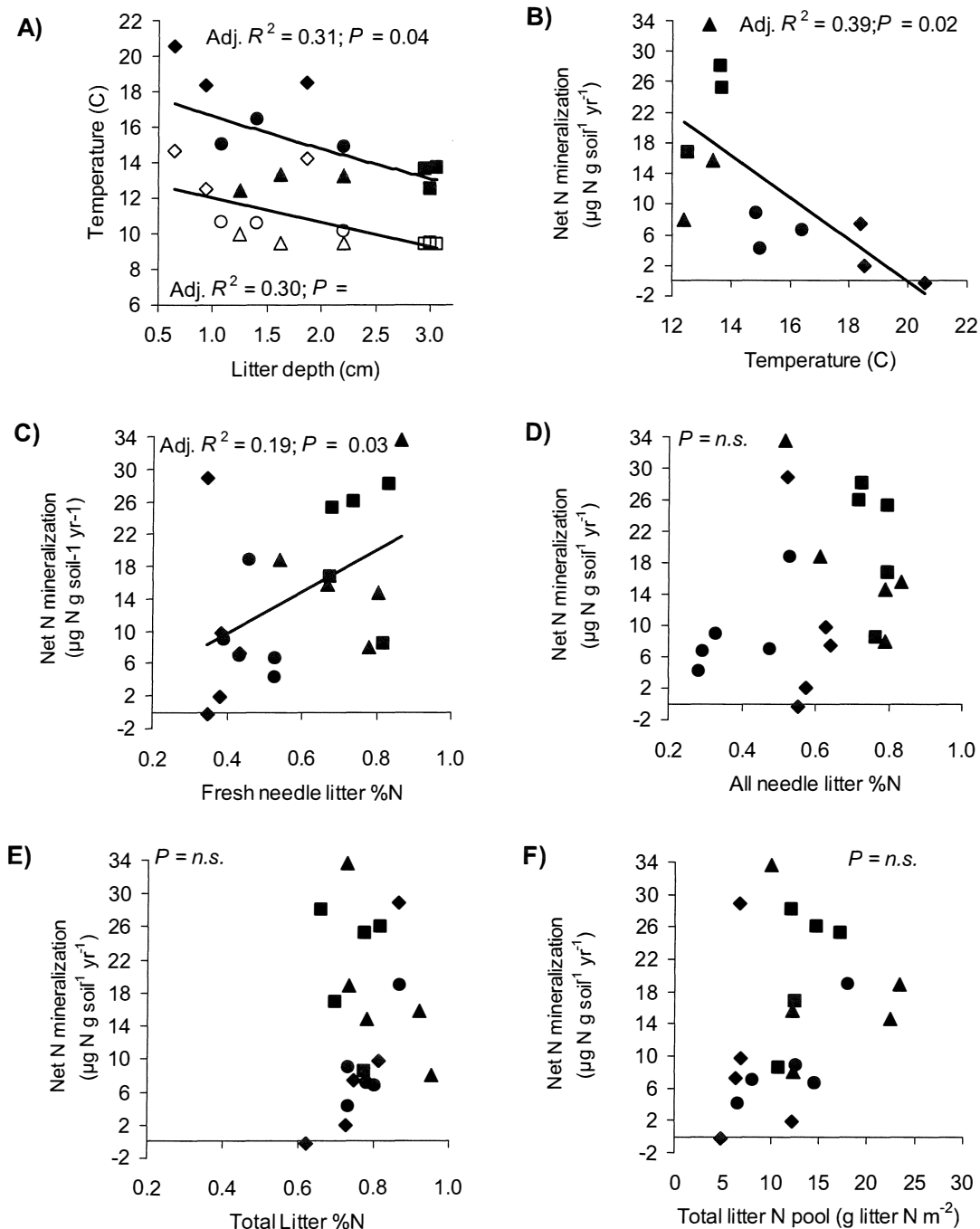
Fig. 5. Relationships between litter depth and N content, soil temperatures, and net N mineralization rates across a chronosequence of mountain pine beetle disturbance in lodgepole pine. ● = undisturbed, ■ = red stage, ▲ = gray stage, ◆ = 30 year after outbreak. (A) Soil temperature vs. litter depth. Solid symbols = litter–soil interface temperatures, open symbols = 10-cm soil depth temperatures; (B) net N mineralization vs. litter–soil interface temperature; (C–E) net N mineralization vs. fresh needle litter %N (C), all needle litter %N (D), and total litter %N (E); (F) net N mineralization vs. litter N pool. In panels A and B, n = 12 as only three plots per class were instrumented with temperature probes; All plots are included in panels C–F ( n = 20 ). Summary statistics and regression lines in each panel are for significant linear regressions.
