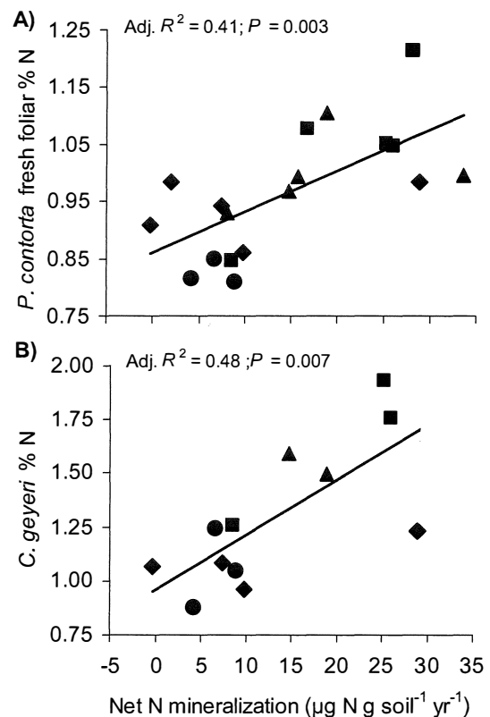
Fig. 6. Foliar %N of unattacked lodgepole pine (A) and %N of the sedge Carex geyerii (B) vs. soil N mineralization rate in a chronosequence of mountain pine beetle disturbance in lodgepole pine. ● = undisturbed, ■ = red stage, ▲ = gray stage, ◆ = 30 year after outbreak. Summary statistics are from linear regression.
