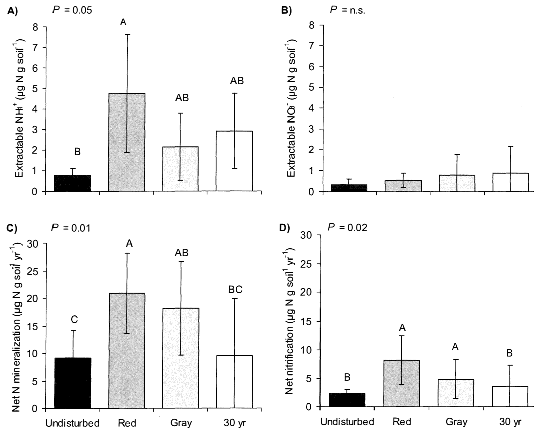
Fig. 4. Soil N pools and fluxes across a chronosequence of mountain pine beetle disturbance in lodgepole pine. For extractable \text{NH}_4^+ pool size (panel A), and extractable \text{NO}_3^- pool size (panel B), significance levels are from ANOVA and Tukey's HSD test ( \alpha = 0.05 ). For net mineralization rate (panel C), and net nitrification rate (panel D), significance levels were determined from general linear models reported in Table 3. Summary statistics in each panel are for the class terms in each respective model, and values within the same panel with the same letter are not significantly different. Error bars = 2 standard errors.
