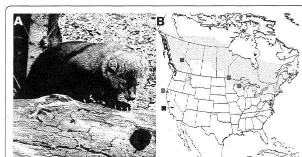
Figure 1 North American fisher and its geographic distribution. Fisher ( Martes pennanti ), a mid-sized carnivore, is distributed throughout boreal and montane North America. Subspecific classification has followed geographic subdivision of this range: ssp. pennanti occurs in the east (blue), ssp. columbiana occurs in the Northern Rocky Mountains (light and dark green), and ssp. pacifica is found along the Pacific coast (light and dark red).
