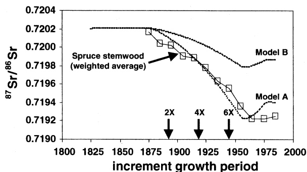
Figure 9. Results of mass balance model describing evolution of ^{87}\text{Sr}/^{86}\text{Sr} of the forest floor in response to changing atmospheric deposition of Sr. Sr deposition was assumed to be equal to the 'baseline' value (present-day Sr deposition flux) from 1825 to 1875. Beginning in 1875, Sr deposition was increased annually by a set increment, reaching a maximum in 1955. After 1955, Sr deposition was decreased annually by a set increment, returning to the baseline value in 1975. Curve labeled 'model A' shows result when the maximum deposition value was adjusted to give agreement between model results and the trend of weighted average spruce stemwood compositions (Table 2; open squares). 'X-factor' arrows show year in which Sr deposition for this model reached 2 times, 4 times and 6 times baseline levels. Curve labeled 'model B' shows result when the maximum deposition value was taken to be that measured at Hubbard Brook watershed from 1963 to 1966 (Likens et al. 1998).
