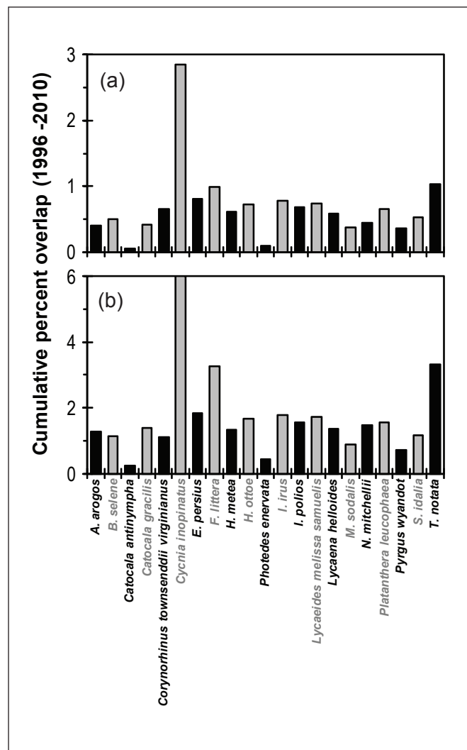
Figure 7.—Cumulative percentage of overlap between each species' known distributional range and (a) the actual area treated with Btk and (b) the actual treated area including 1 x 1-km overlapping cells.
