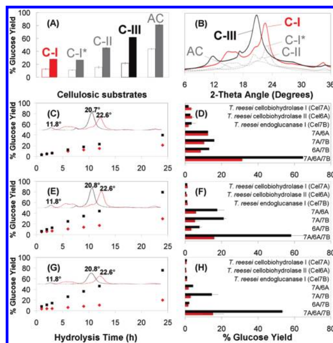
Figure 3. Enzymatic digestibility of cellulose as a function of its crystalline state and cellulases employed. (A) Native cellulose (cellulose I β , or C-I), derived from Avicel, was treated with liquid ammonia (cellulose III I , or C-III), sodium hydroxide (cellulose II, or C-II), 28% ammonium hydroxide (C-I*), and concentrated phosphoric acid (amorphous cellulose, or AC). Equivalent enzyme loadings were added for each assay (1.5 FPU Spezyme CP cellulase/g glucan + 6.4 p-NPGU Novo188 \beta -glucosidase/g glucan). The left and right bars represent 6 and 24 h data, respectively. (B) XRD spectra for cellulose allomorphs ( 2\theta range 6°–36°). (C–H) Hydrolysis time course for cellulose I β (red diamonds) and cellulose III I (black squares) derived from Avicel (C), cotton linters (E), and cotton fibers (G). Inset depicts XRD spectra for respective substrates. Avicel was hydrolyzed by \sim 1.5 FPU Spezyme CP cellulase/g glucan, while the cotton-derived substrates were hydrolyzed by \sim 15 FPU Spezyme CP cellulase/g glucan. Enzymatic digestibility of cellulose I β (red bars on bottom) and cellulose III I (black bars on top) derived from Avicel (D), cotton linters (F), and cotton fibers (H) for various combinations of T. reesei -based exo- (Cel7A, Cel6A) and endoglucanases (Cel7B). Equivalent enzyme loadings were added for each assay (2.5 mg of each cellulase/g Avicel or 10 mg of each cellulase/g cotton-derived substrates). In each case, 10% additional \beta -glucosidase relative to total cellulase was added to prevent cellobiose buildup.
