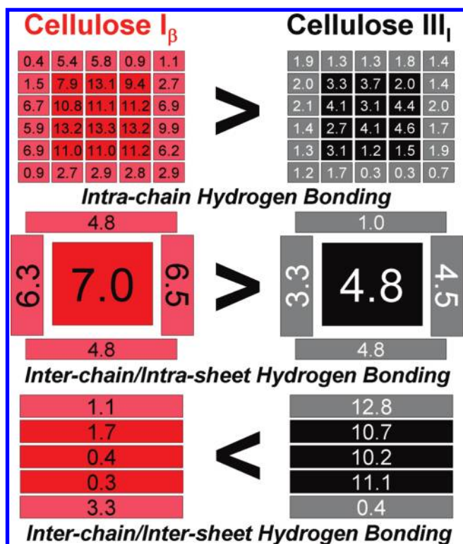
Figure 2. Hydrogen bond network in cellulose I β (left) and cellulose III I (right). The two 6 × 5 grids on the top row show the average number of intrachain HBs per chain. The central row shows the average number of “interchain/intrasheet” HBs (HBs between glucan chains within the same fibril horizontal layer), while the bottom row shows the average number of “interchain/intersheet” HBs (HBs between neighboring layers within the cellulose fibril). The crystalline core (dark red or black) and solvent-exposed (pink or gray) cellulose chains are highlighted.
