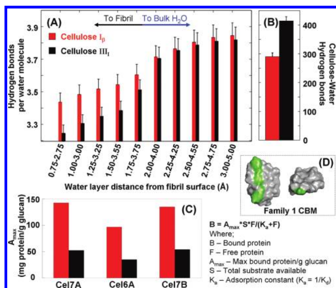
Figure 5. Influence of cellulose I_{\beta} (red bars, left) and cellulose III_I (black bars, right) crystal structures on fibril hydration and cellulase binding capacity. Average number of hydrogen bonds between water molecules (A) and between cellulose–water molecules (B) in the vicinity of cellulose I_{\beta} and III_I fibril surfaces as predicted by MD simulations. (C) Maximum T. reesei exo- and endocellulases' binding capacity determined from Langmuir adsorption model for 277 K equilibrium adsorption to cellulose I_{\beta} and cellulose III_I . (D) Family 1 cellulase binding module bottom (left) and side views (right) (PDB code: 1CBH), with aromatic residues highlighted in green. Protein structure generated using Pymol. 45
