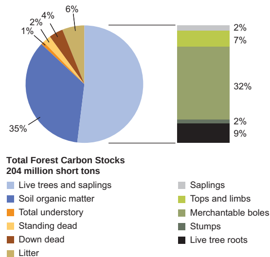
Figure 29. —Estimated total carbon stocks on forest land by component, Maryland, 2008.
