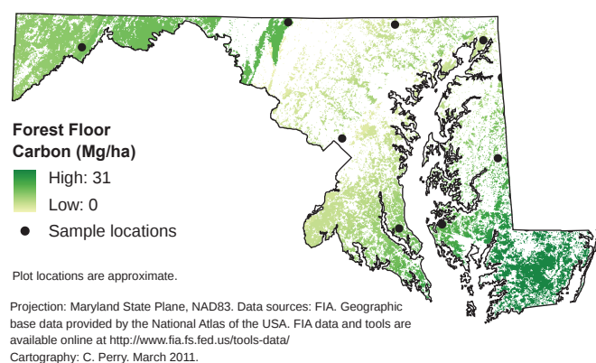
Figure 72. —Modeled forest floor carbon storage (Mg/ha), Maryland, 2004-2006.
