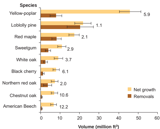
Figure 45. —Average annual net growth, removals, and growth-to-removals (G:R) ratio for major species, Maryland, 2008. G:R for all species is 2.6. (Error bars show 68 percent confidence intervals around the mean.)
