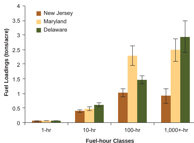
Figure 61. —Means and associated standard errors of fuel loadings (tons/acre, time-lag fuel classes) on forest land in Maryland and neighboring states, 2008. (Error bars show 68 percent confidence intervals around the mean.)
