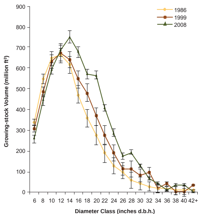
Figure 36. —Growing-stock volume on timberland by diameter class and inventory year, Maryland, 1986, 1999, 2008. (Error bars show 68 percent confidence intervals around the mean.)
