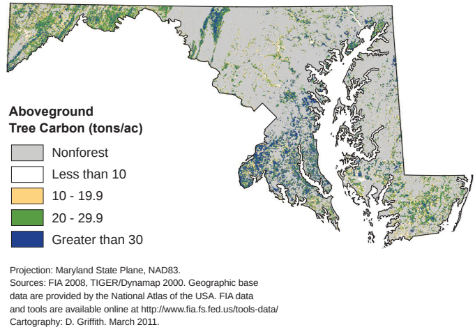
Figure 28. —Distribution of aboveground live tree carbon in Maryland, 2008.
