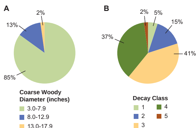
Figure 62. —Mean percentage of coarse woody debris pieces per acre by transect diameter (inches) (A) and decay classes (B) on forest land in Maryland, 2008.
