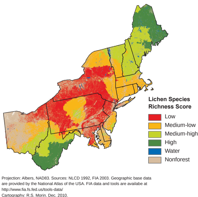
Figure 66. —Estimated lichen species richness, northeastern U.S., 2000-2003.
