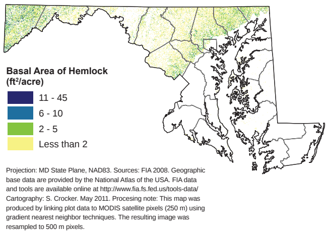
Figure 83.—Distribution of hemlock on forest land, Maryland, 2008.
