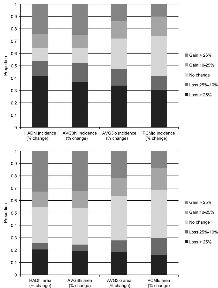
Figure 4. Change in species area-weighted incidence and total area occupied in the eastern US based on shifts in suitable habitat under four climate change scenarios.
