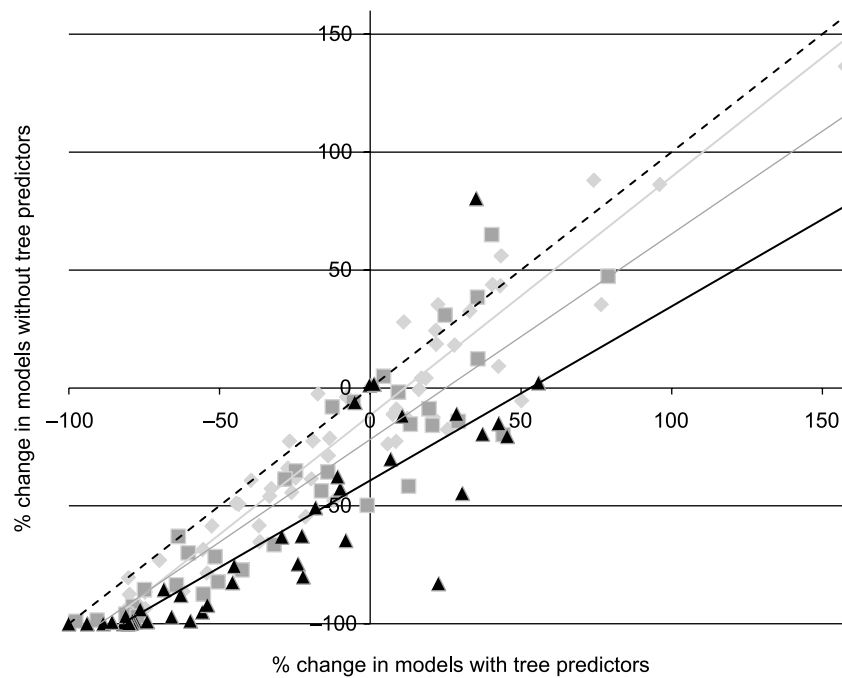
Figure 7. Projected change in habitat for species with and without vegetation variables in the predictor set. Black triangles indicate models where there were two or three tree species in the top three variables, dark gray squares indicate only one variable in the top three, and light gray diamonds indicate species models without tree species in the top three variables. Lines of the same shading are simple linear regressions by groupings with no tree species, one tree species, and > two tree species in top three variables with r^2 values of 0.94, 0.90, and 0.86, respectively, and the dashed 1:1 line for reference. Ten species have changes >160% and are not shown.
