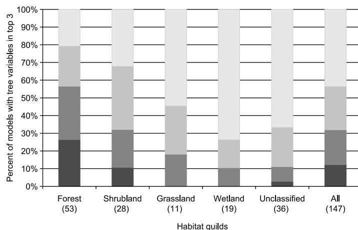
Figure 2. The occurrence and number of tree species variables in the three most influential variables in each bird species model, separated by bird habitat guild. Number in parentheses indicates the number of species models within that habitat guild.
