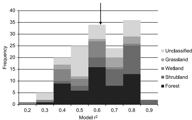
Figure 1. Predictive model fit of randomForest models (equivalent to r^2 ) for 147 bird species, as classified by a priori habitat characteristics. Arrow indicates the mean model r^2 across all species (0.66).
