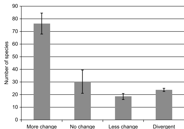
Figure 6. The mean number of species from the four scenarios (with SD) in which the species model without vegetation resulted in a greater projection of change, no change, less change, or divergent results from the species model when tree species were in the pool of predictor values.
