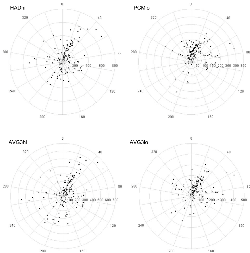
Figure 5. Potential changes in distance (km) and direction (degrees) of mean-centers of suitable habitat for 147 species for AVG3lo (note distance scale from 0 to 500 km), PCMIo (0–350 km), AVG3hi (0–700 km), and HADhi (0–800 km).
