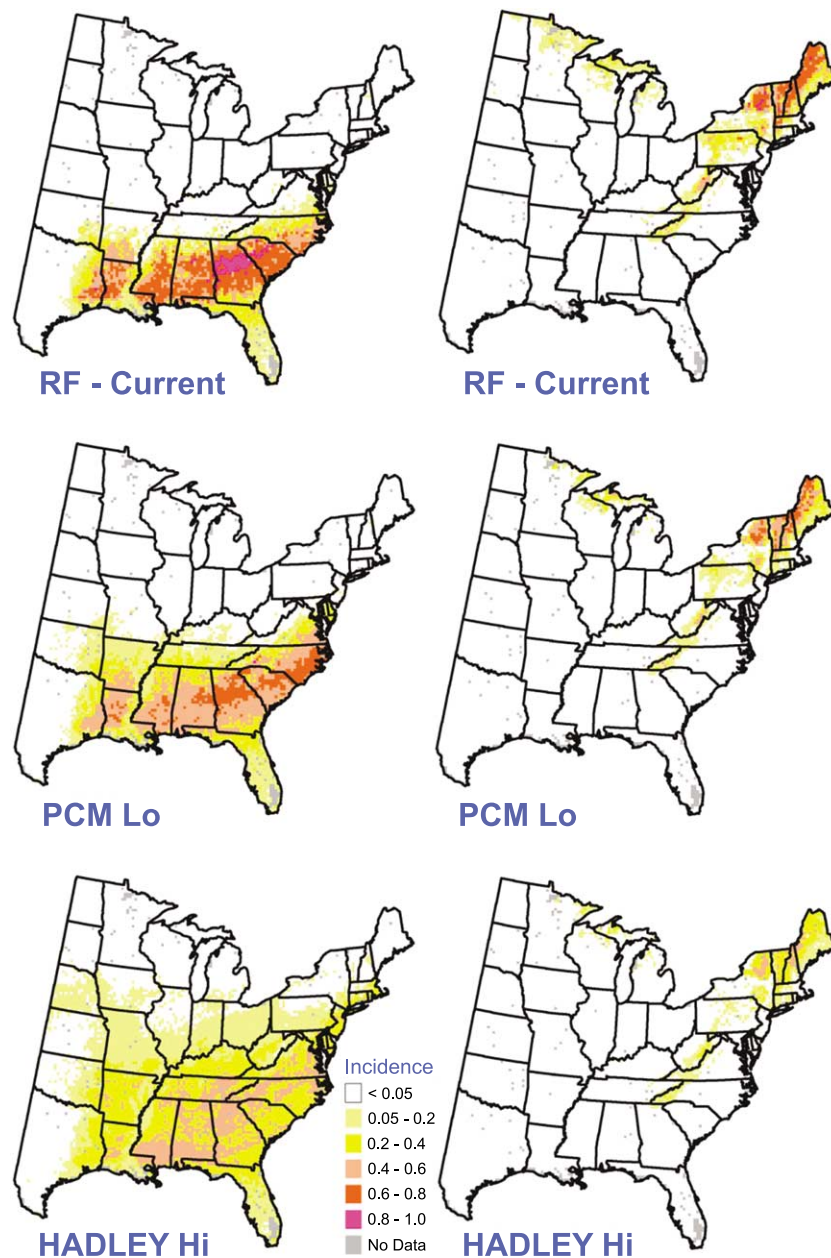
Figure 3. The current modeled distribution (RF-current) of the brown-headed nuthatch (left column) and black-throated blue warbler (right column) and projected suitable habitat under HADhi and PCMlo climate change scenarios.
