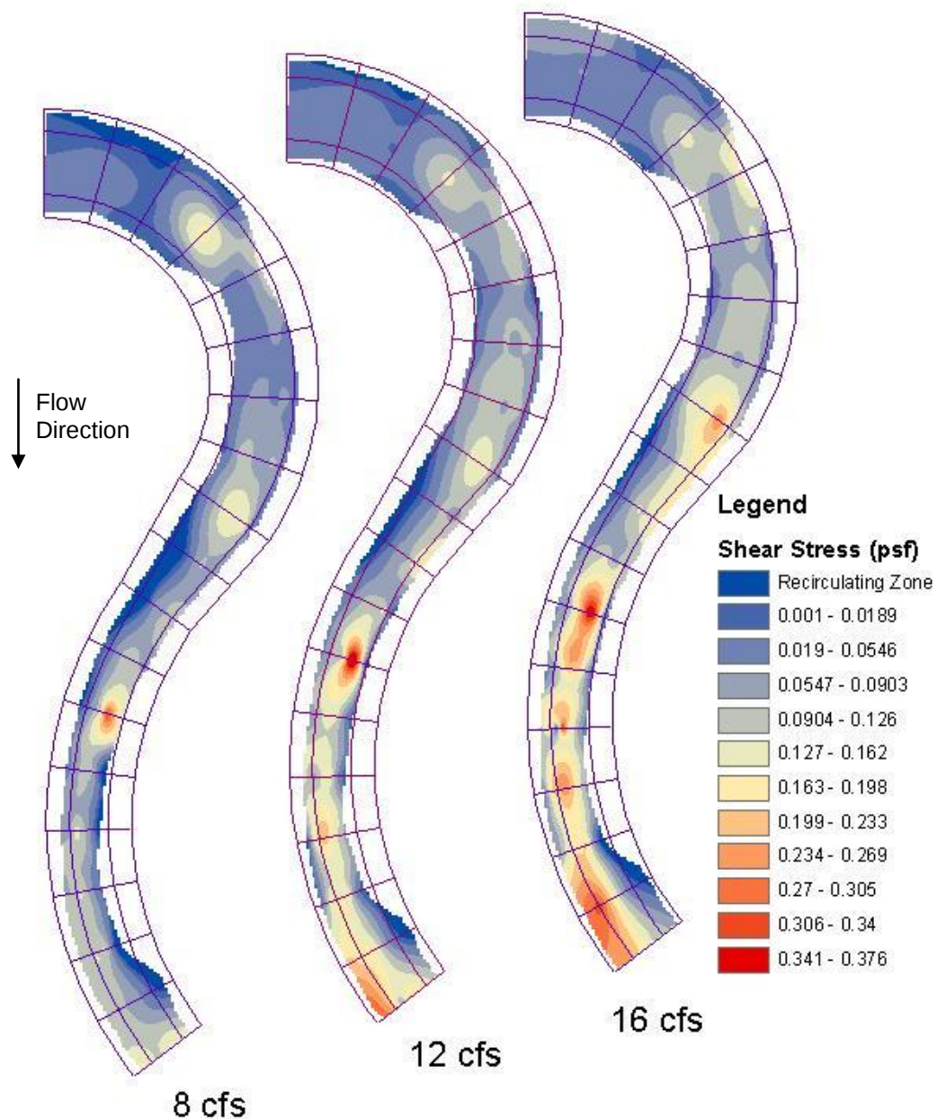
Figure 5-6: Preston tube shear stress distributions per discharge
