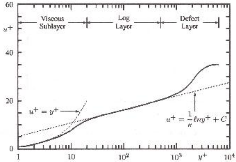
Figure 2-12: Regions identified in the velocity profile where u^+ = v_x/u_* and y^+ = u_*y/\nu (Wilcox, 2007)
