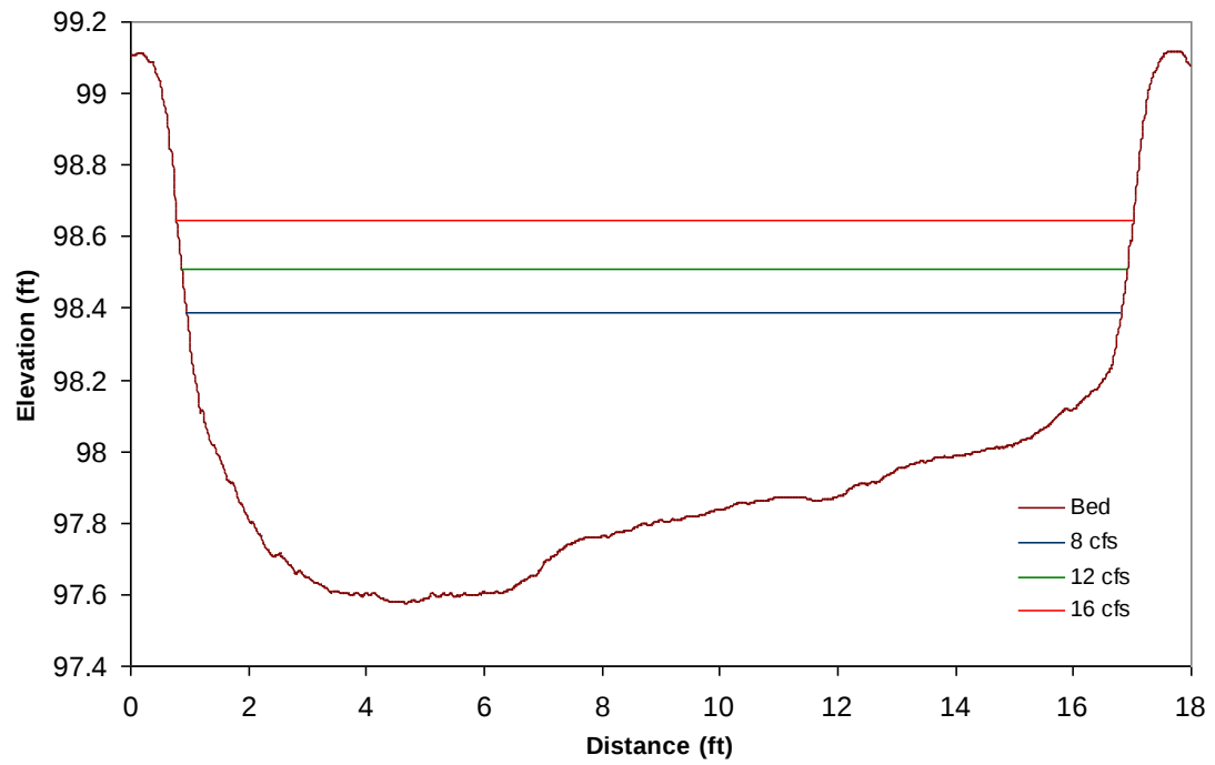
Figure A-1: Cross section 1
