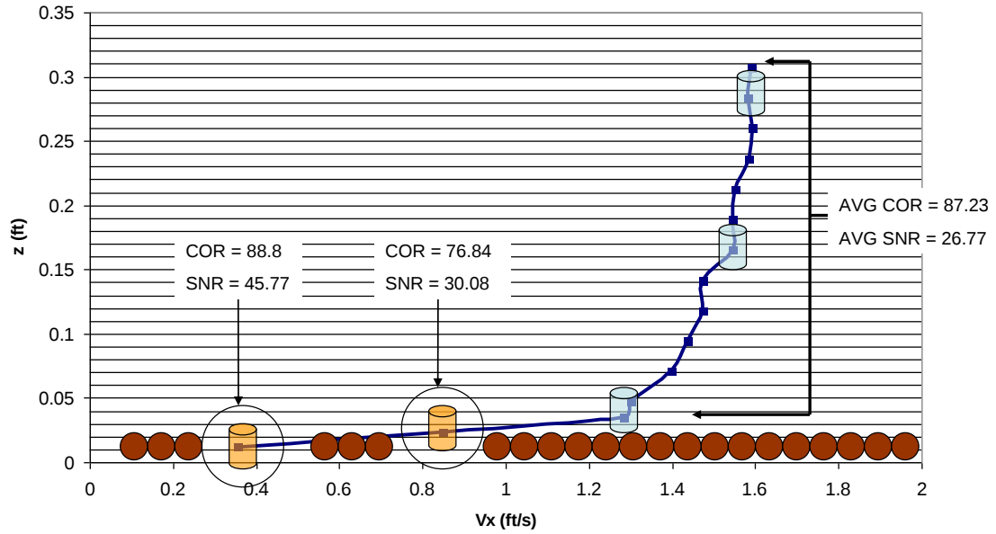
Figure 4-5: SNR for near-bed ADV measurements
