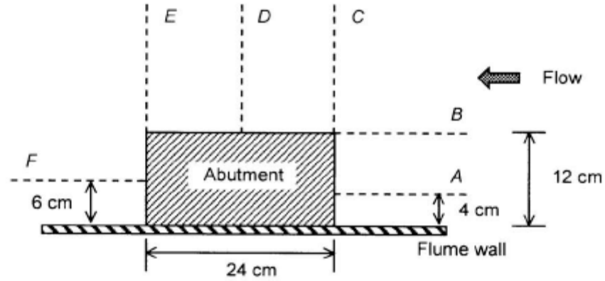
Figure 2-16: Measurement sections around abutment (Dey and Barbhuiya, 2005)
