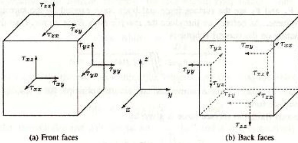
Figure 2-14: Stresses acting on a fluid body (Wilcox, 2007)
