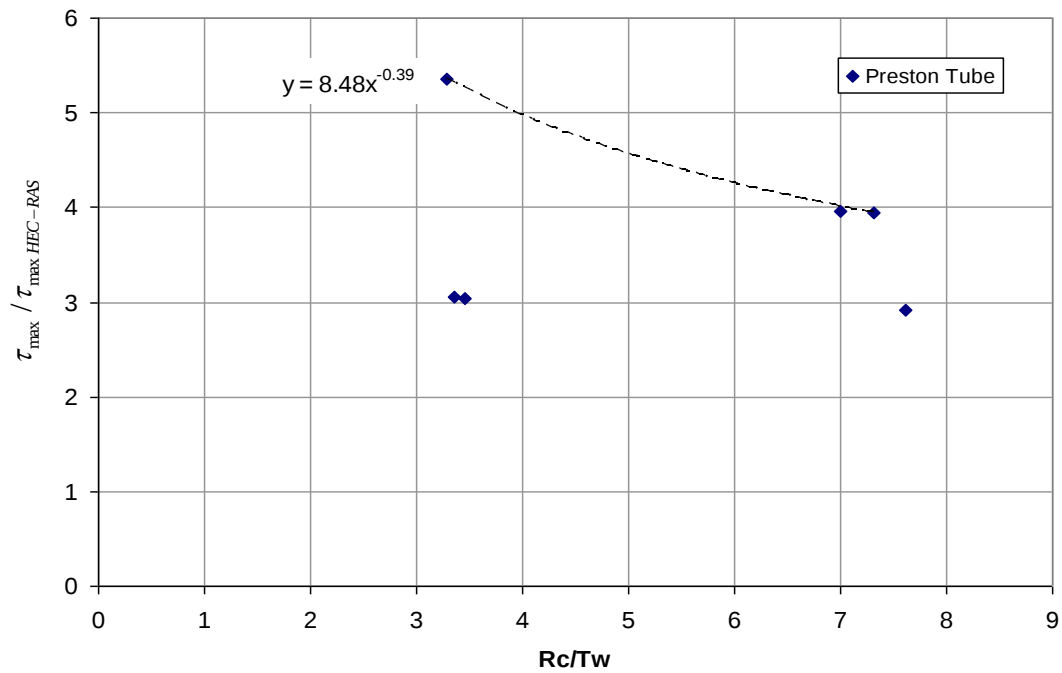
Figure 6-13: Comparison of bend maximums from HEC-RAS
