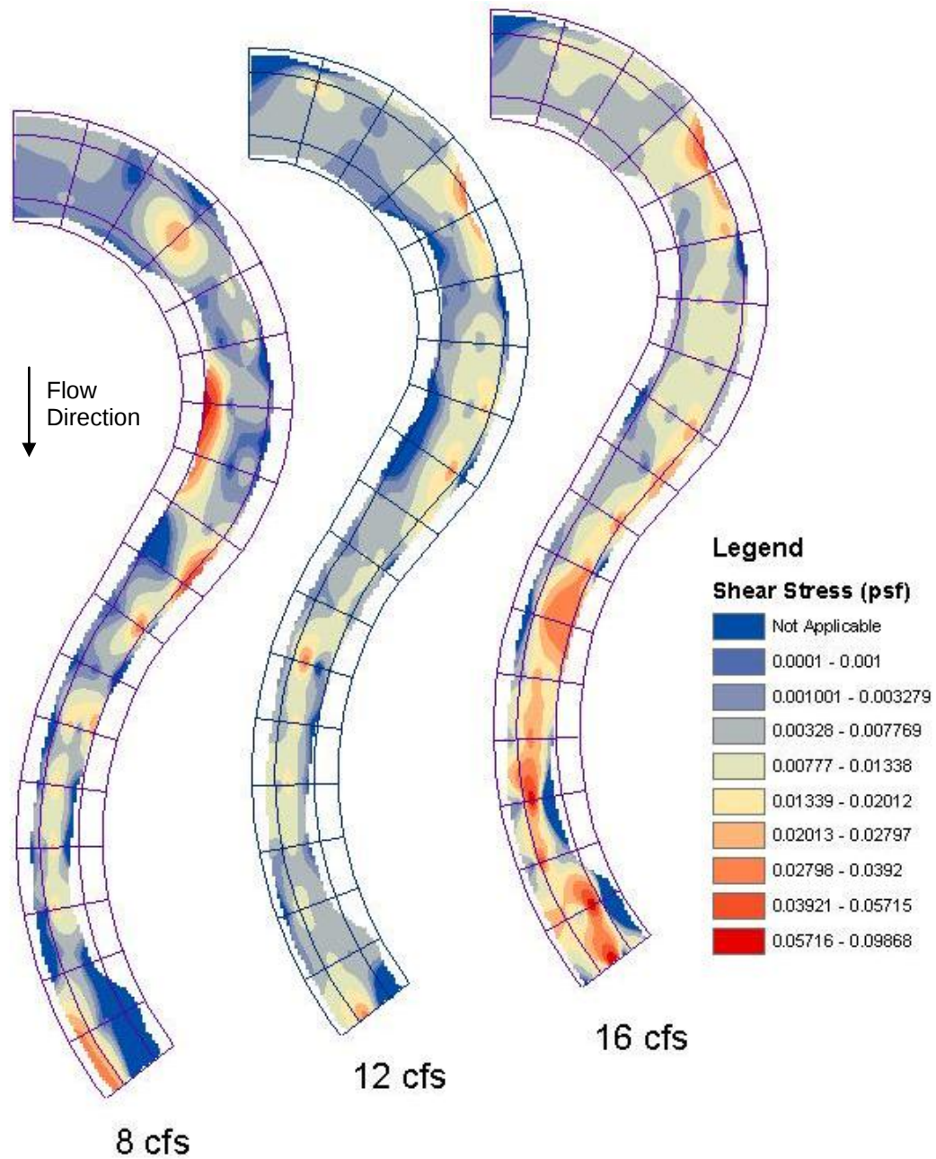
Figure 5-20: Shear stress distributions by the TKE method
