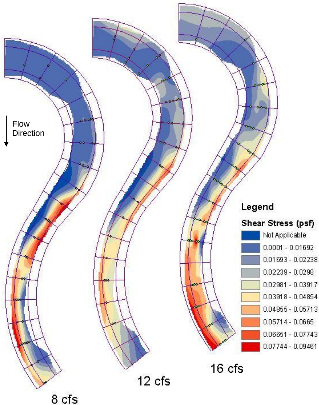
Figure 5-18: Shear stress distributions for Reynolds – extrapolation technique
