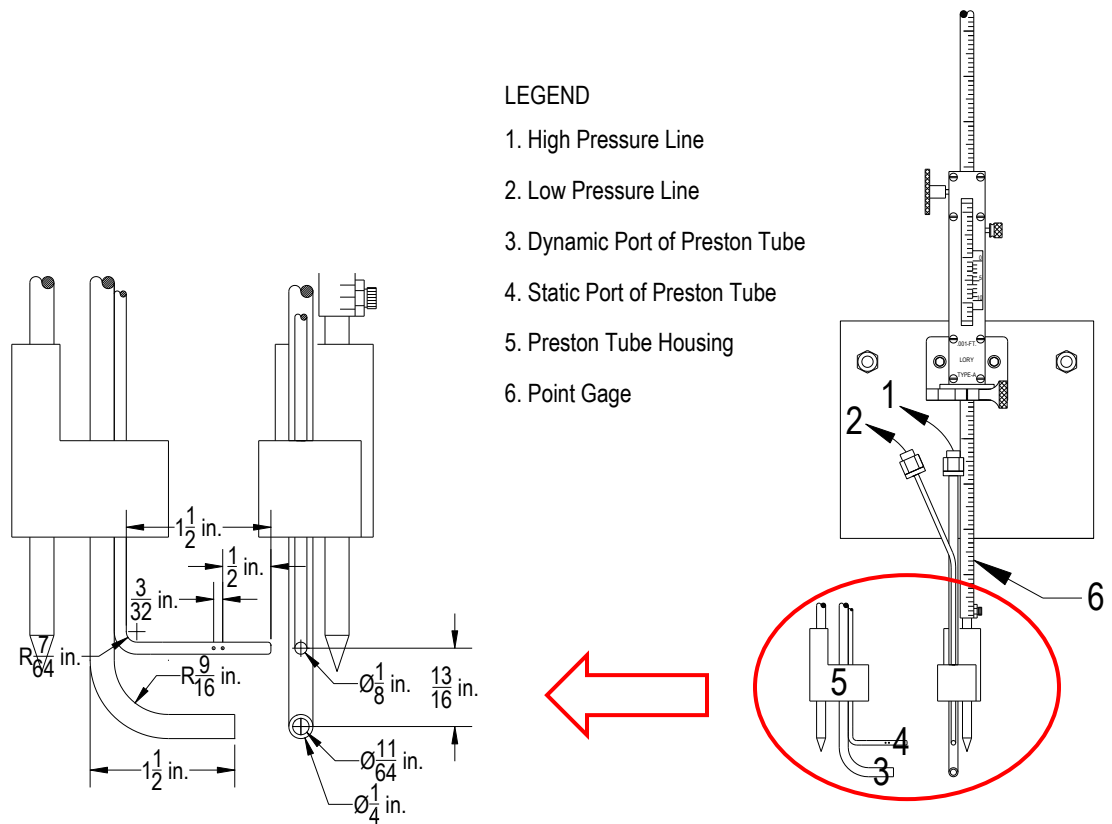
Figure 3-5: Preston tube schematic (Sclafani, 2008)
