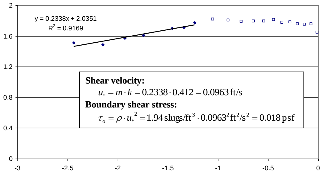
Figure 5-11: Regression of logarithmic profile for 16 cfs at Cross section 6, Location b
