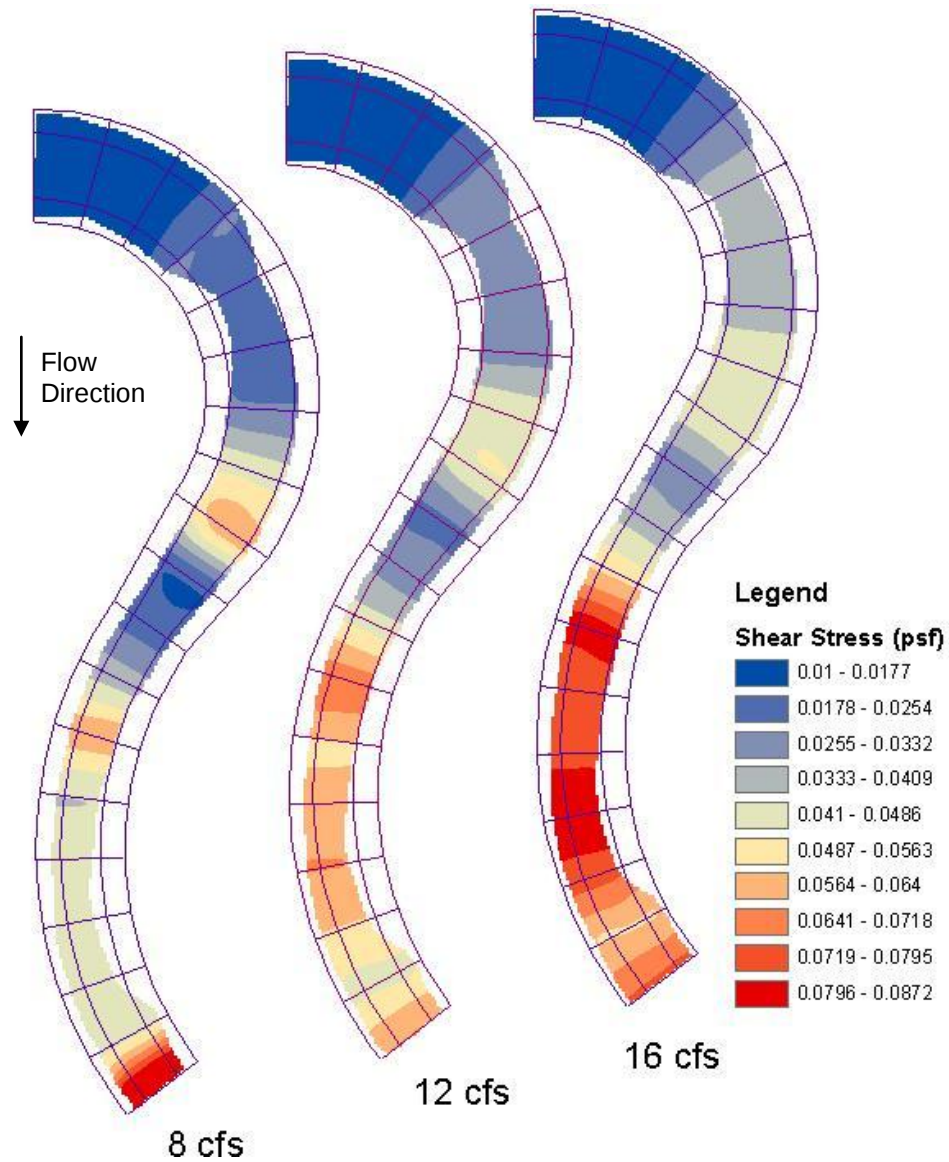
Figure 5-5: HEC-RAS shear stress distribution per discharge
