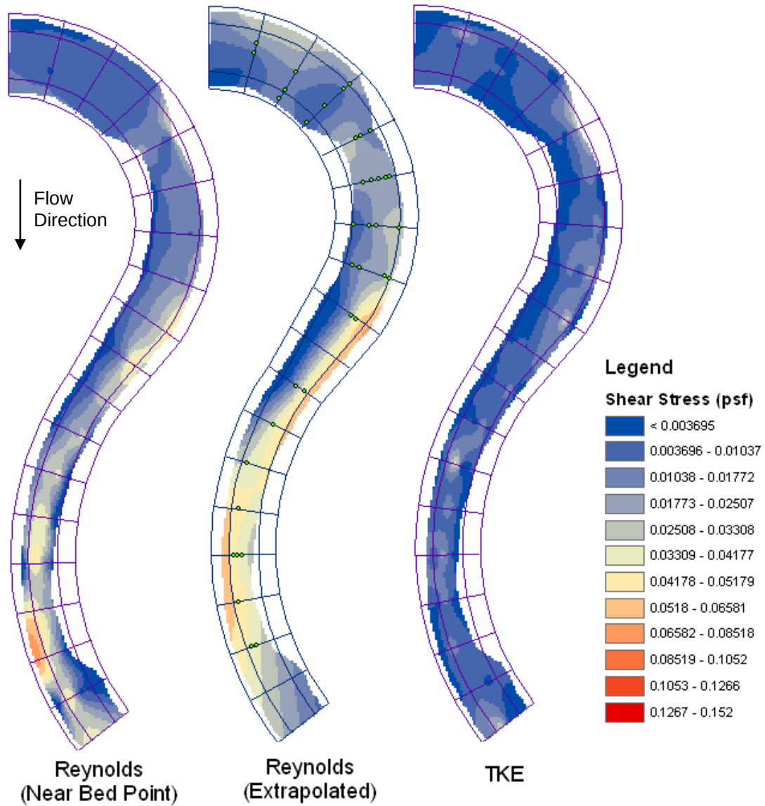
Figure 6-8: Comparisons between Reynolds and TKE methods (12 cfs)
