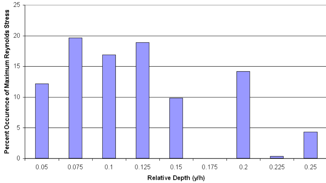
Figure 5-14: Percent occurrence of maximum Reynolds stress -\overline{\rho u'w'} per measured relative depth
