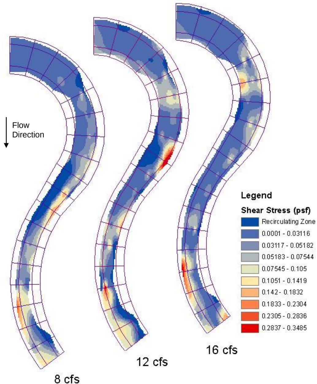
Figure 5-13: Law of the wall shear stress distributions per discharge
