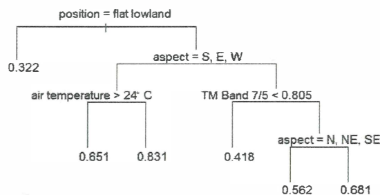
Fig. 2. Decision tree model for relative organic layer depth reduction.
