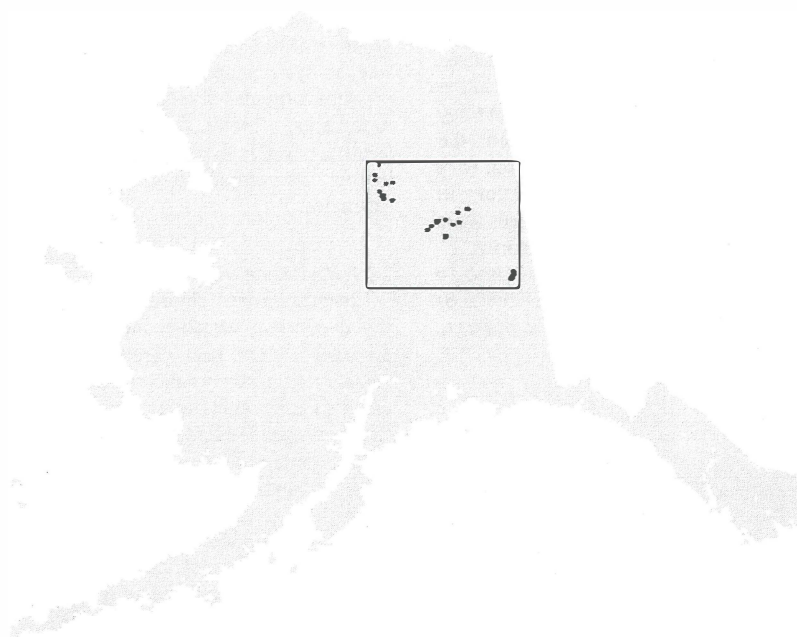
Fig. 1. Study area of the Alaskan interior, points mark the locations of burn depth observations.
