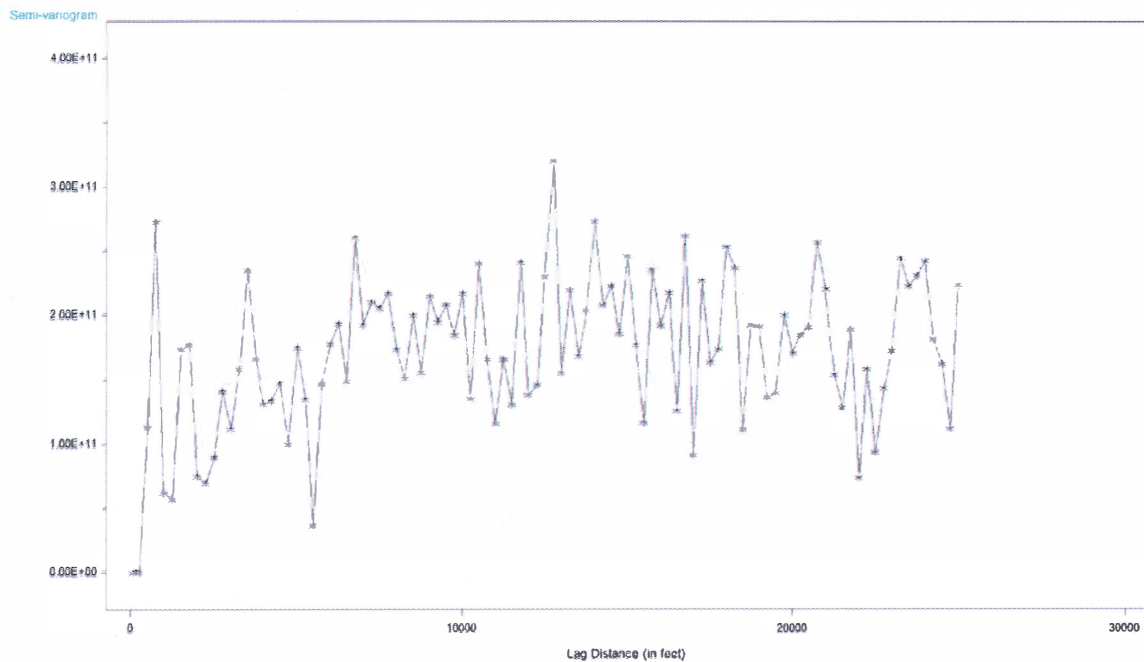
Fig. 2. Semivariogram of regression model residuals.
