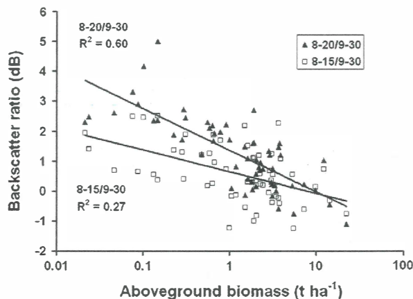
Fig. 4. Variations in the L-HV backscatter ratio ( \sigma^0_r ) between wet and dry dates as a function of aboveground biomass. R^2 values are significant at p < 0.0001 . (8-20/9-30 denotes that the backscatter ratio between 20 August 2009 [moderate moisture] and 30 September 2007 [very high moisture]. 8-15/9-30 denotes the backscatter ratio between 15 August 2007 [high moisture] and 30 September 2007 [very high moisture].).
