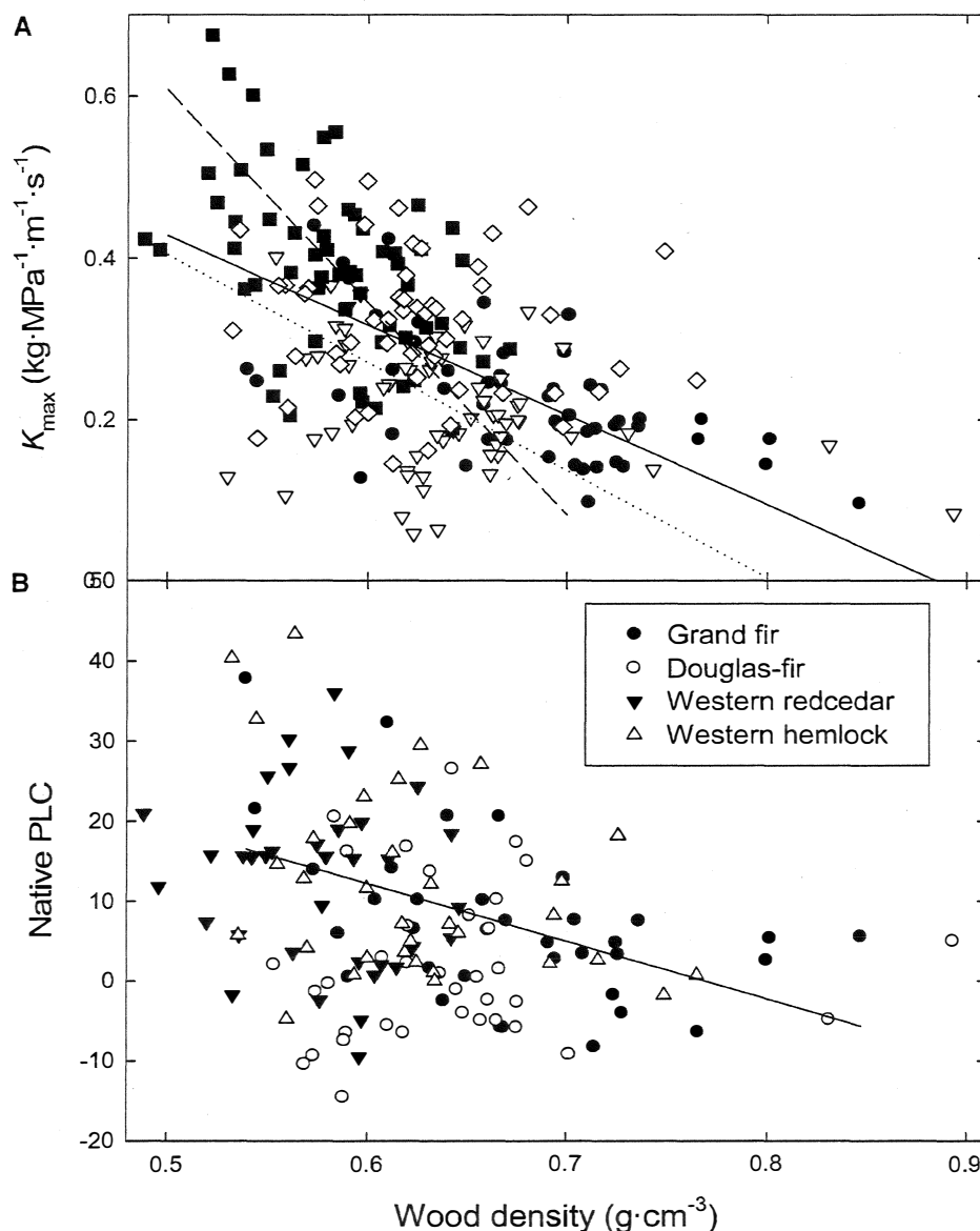
Fig. 3. (A) Maximum specific conductivity ( K_{\max} ) and (B) native percent loss of conductivity (PLC) of small diameter branches vs. their wood density for four conifer species. The native PLC values are only from months without freeze-thaw events. In (A), significant relationships (SMA P < 0.03 ) were found in grand fir (solid line), Douglas-fir (dotted line) and western redcedar (dashed line), but not western hemlock. In (B), a significant relationship (SMA P = 0.016 ) was found only for grand fir.
