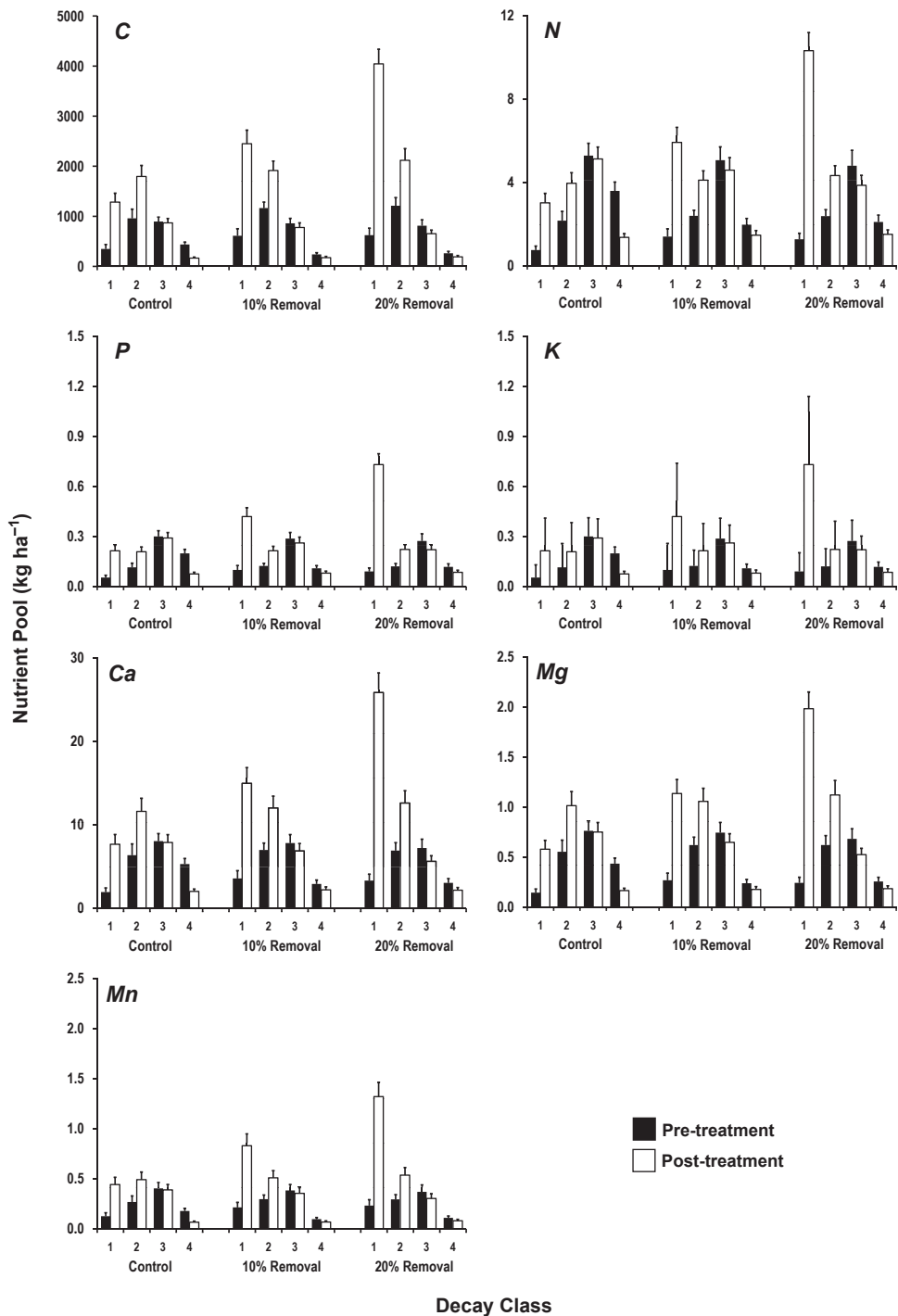
Fig. 3. Mean stand-level nutrient pool of down woody debris, as separated by decay class, before and after harvest. Bars indicate +1 standard error. Means and standard errors are calculated from only those plots within the three replicates for that particular treatment.
