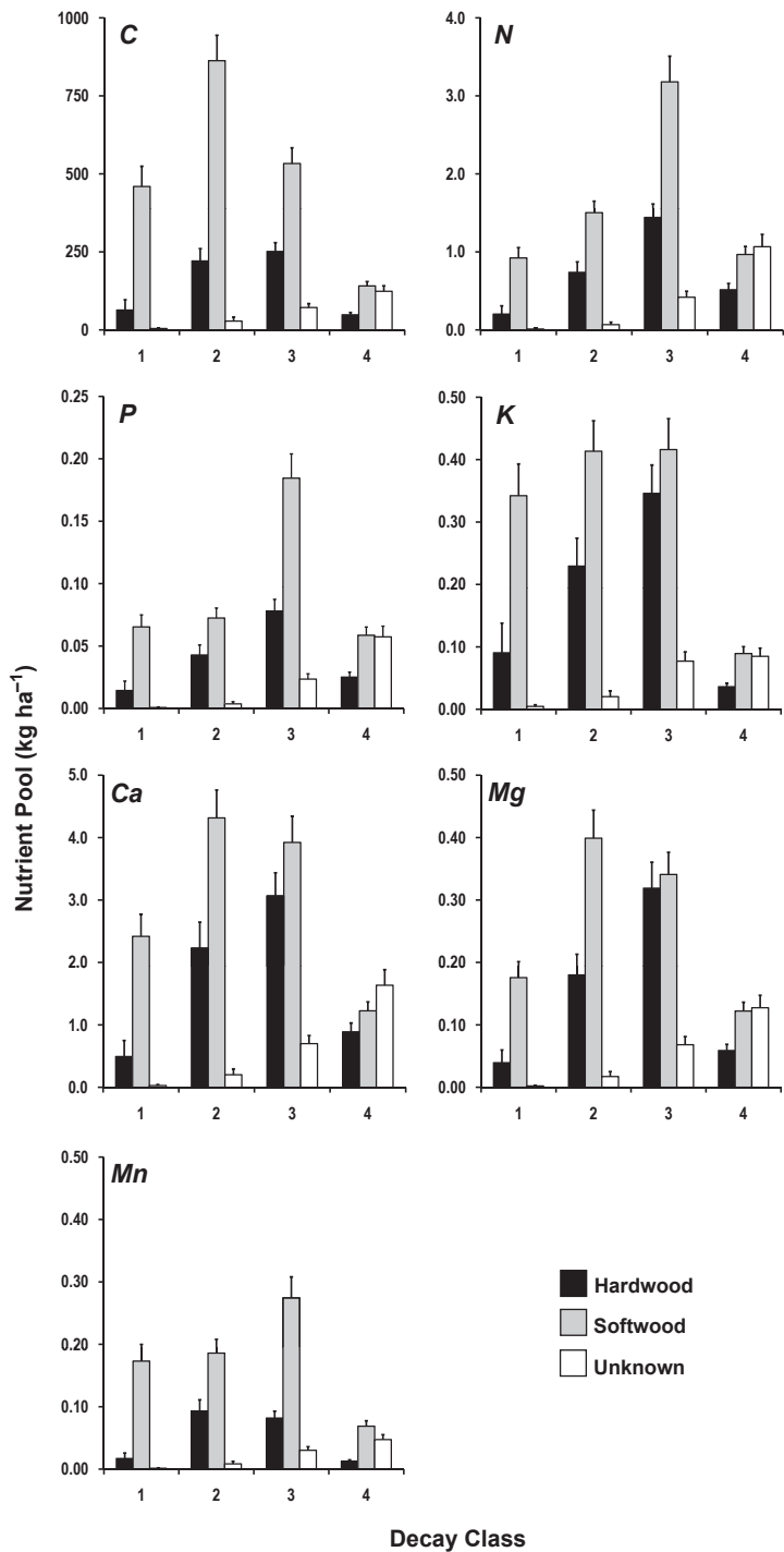
Fig. 2. Mean stand-level nutrient pool of down woody debris, as separated by wood type (hardwood vs. softwood) and decay class, before harvest in 1995. Bars indicate +1 standard error. Means and standard errors are calculated from volume estimates pooled across all replicates (Fraver et al. 2002).
