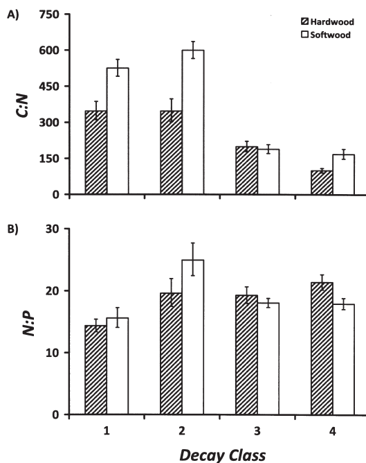
Fig. 1. Mean A) carbon-nitrogen (C:N) and B) nitrogen-phosphorus (N:P) ratios for each decay class for hardwood and softwood down woody debris. Bars indicate \pm 1 standard error.
