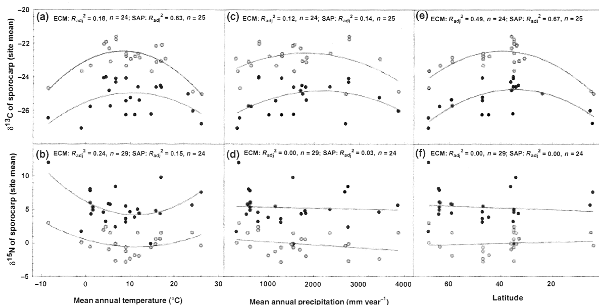
Figure 3 Regressions of site mean fungal \delta^{13}\text{C} and \delta^{15}\text{N} values with mean annual temperature, mean annual precipitation, and latitude. Black circles are site means of ectomycorrhizal (ECM) fungi; grey circles are site means of saprotrophic (SAP) fungi. Linear vs. quadratic best-fit polynomial equations were compared and equations producing the best R^2 coefficient are presented. Tanigawa and Okinawa, Japan, sites were removed from graphs (b, d, f) as statistical outliers. Equations of lines: (a) f_{\text{SAP}} = -23.02 + 0.14(x) - 0.01(x)^2 , f_{\text{ECM}} = -25.49 + 0.11(x) - 0.005(x)^2 ; (b) f_{\text{SAP}} = 0.53 - 0.19(x) + 0.008(x)^2 , f_{\text{ECM}} = 6.22 - 0.36(x) - 0.016(x)^2 ; (c) f_{\text{SAP}} = -23.8 + 0.1E^{-2}(x) - 3.9E^{-007}(x)^2 , f_{\text{ECM}} = -26.57 + 0.002(x) - 3.8E^{-007}(x)^2 ; (d) f_{\text{SAP}} = 0.69 - 0.5E^{-3}(x) , f_{\text{ECM}} = 5.55 - 0.2E^{-3}(x) ; (e) f_{\text{SAP}} = -25.56 + 0.16(x) - 0.002(x)^2 , f_{\text{ECM}} = -26.81 + 0.12(x) - 0.002(x)^2 ; (f) f_{\text{SAP}} = 0.35 - 0.01(x) , f_{\text{ECM}} = 4.69 + 0.01(x) .
