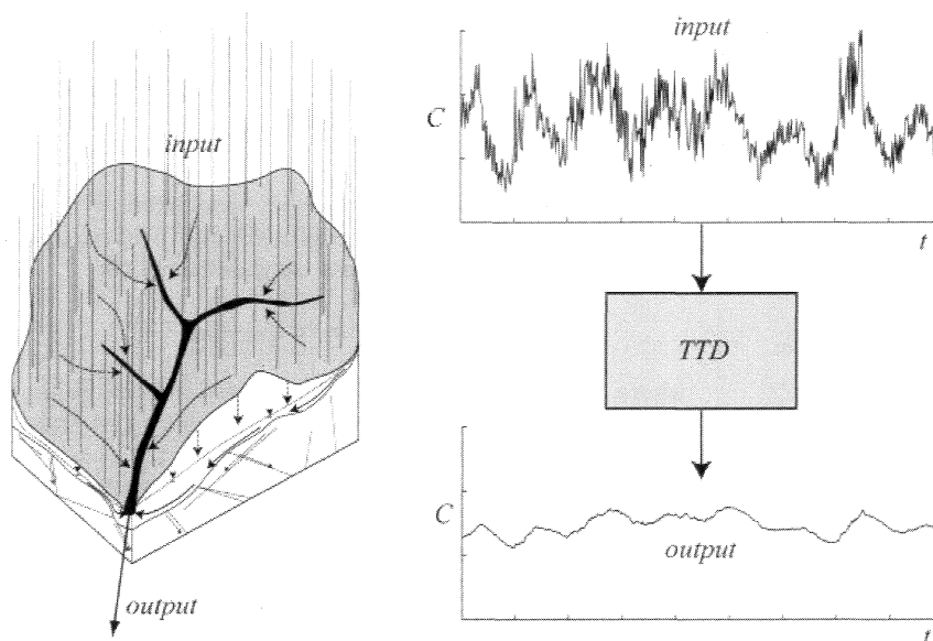
Figure 1. Schematic illustrating that spatially distributed inputs received by a catchment travel along heterogeneous flow paths to the catchment outlet (output). The diagram shows how a conservative tracer input to a catchment will be 'filtered' as the water passes through the system to the catchment outlet, yielding a damped and lagged signal with less high-frequency variation. The transit time distribution (TTD) describes the filtering process
