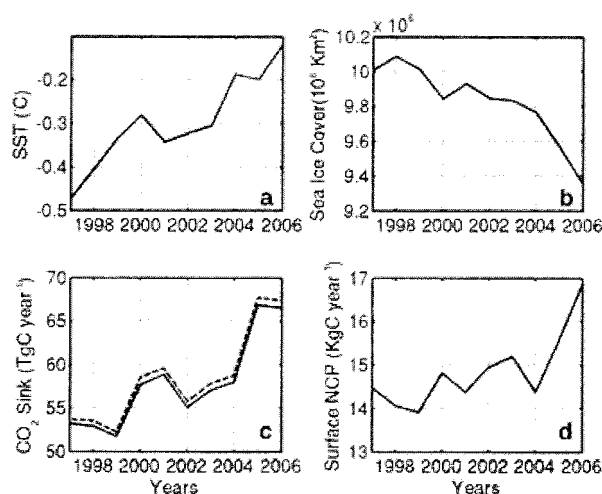
Fig. 8. Annual mean (a) sea surface temperature, (b) sea-ice covered area, (c) \text{CO}_2 oceanic sink (solid line is for climatological DOC inputs and dashed line is for TEM DOC inputs) and (d) surface net community production (NCP) for the simulated period 1997–2006. Values are for the oceanic area north of 65^\circ\text{N} .
