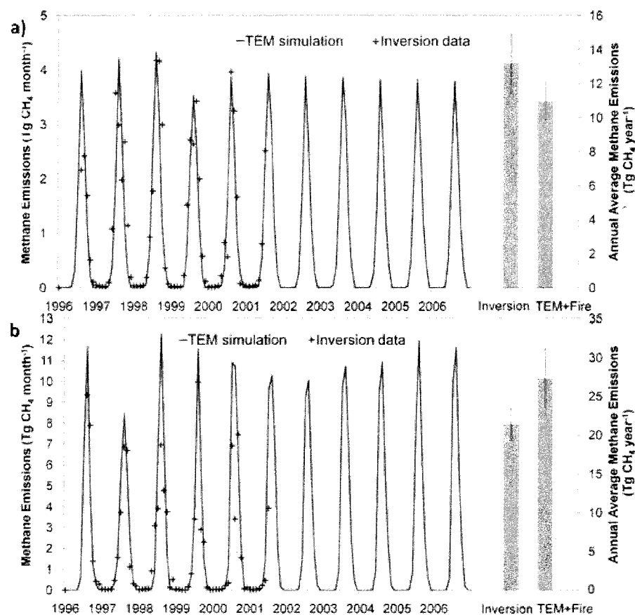
Fig. 6. Comparison \text{CH}_4 exchange estimates between TEM and MATCH simulations in (a) Boreal North America and (b) Boreal Asia: Black solid lines show the seasonal dynamics of biogenic and pyrogenic \text{CH}_4 emissions estimates of TEM from 1996 to 2006 ( \text{Tg CH}_4 per month). Black crosses show the seasonal changes of net \text{CH}_4 emissions from biogenic and pyrogenic sources from 1996 to 2001 estimated by MATCH ( \text{Tg CH}_4 per month). Bars show the annual mean for MATCH simulations (1996–2001) and MDM-TEM simulations (1996–2006) as \text{Tg CH}_4 \text{ yr}^{-1} . Error bars indicate standard deviation (interannual variability) for the time period of the inversion simulations (1996–2001).
