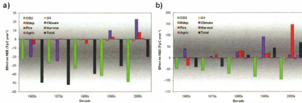
Fig. 11. Total and individual average annual effects ( \text{Tg C yr}^{-1} ) of temporal variability in atmospheric [\text{CO}_2] , tropospheric \text{O}_3 levels, N deposition rates, climate, fire, forest harvest and agricultural establishment and abandonment on NEE for each decade since the 1960s across the Boreal Land Regions in (a) arctic tundra and (b) boreal forest ecosystems.
