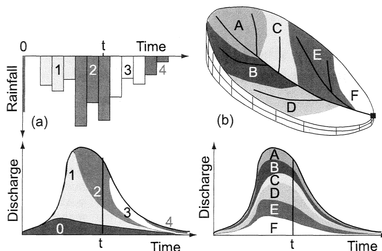
Figure 1. Schematic diagram of our approach; namely the separation of the temporal and spatial hydrograph components. (a) Individual rainfall hyetograph segments are propagated through the storm hydrograph. (b) The geographic source apportionment of flow.
