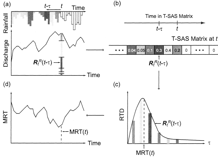
Figure 5. Calculation of mean residence time (MRT) with the T-SAS method. (a) Uses the temporal hydrograph separation developed in Figure 3 to separate the hydrograph into daily values, where R is the percentage of flow from a given precipitation time input at (t - \tau) . (b) The numerical values for the temporal components of flow at time t . (c) Residence time distribution (RTD) for time t calculated using the T-SAS matrix values. (d) Finally, the MRT for the 1-year time series is illustrated schematically showing how the discrete daily MRT calculated from Figure 5c corresponds to other values through the year.
