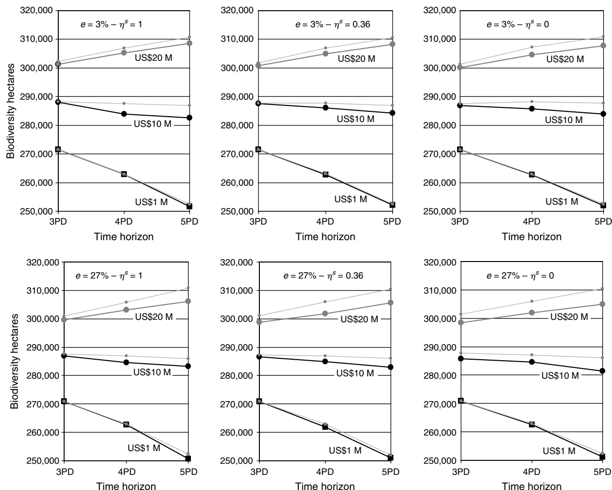
Figure 5. Objective function values (in biodiversity hectares) of best integer solutions and best upper bounds found by the 3-, 4-, and 5-period models at the end of their respective planning horizons under US$1 M, $10 M, and $20 M annual budgets with six supply elasticity and amenity premium combinations.
