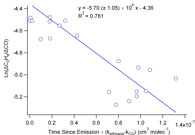
Fig. 6. \ln(\Delta\text{ethylene}/\Delta\text{CO}) vs. time since emission (h) \times (k_{\text{ethylene}} - k_{\text{CO}}) . Average OH in the plume from \sim 10:30\text{--}15:16 LT is initially estimated from the absolute value of the slope ( 5.70 \pm 1.05 \times 10^6 \text{ molec cm}^{-3} ) and then corrected for \text{O}_3 oxidation (see Sect. 3.2.2).
