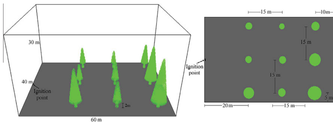
Fig. 3. WFDS simulation design for crown fire initiation showing nine trees with different dimensions but similar CBH (i.e., 2 m).
