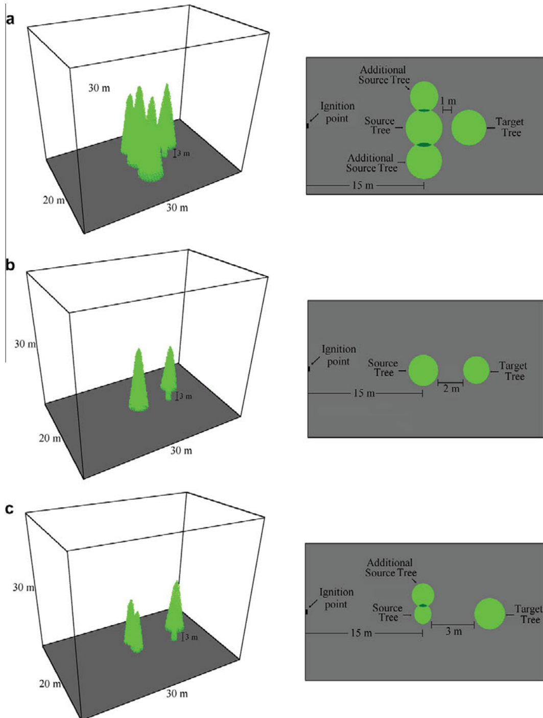
Fig. 4. WFDS simulation design for crown fire propagation. Examples show three, one, and two trees forming the flaming front (a, b, and c) and increasing spacing between the source and target tree.
