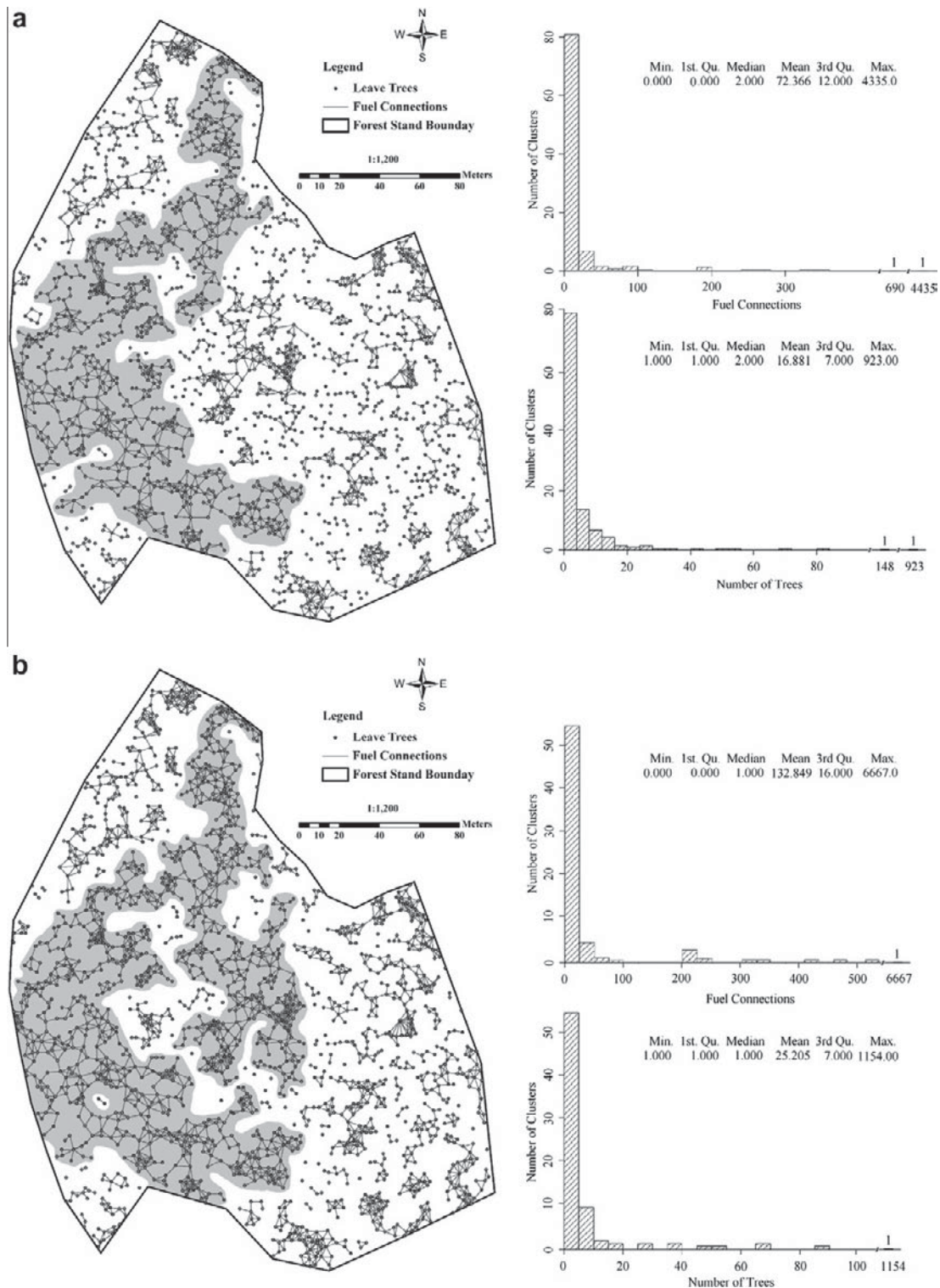
Fig. 8. Location and size of clusters formed by predicted tree-level fuel connections for thinning scenario II under average (a) and severe (b) weather conditions.
