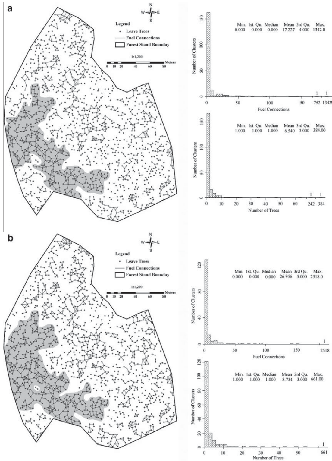
Fig. 9. Location and size of clusters formed by predicted tree-level fuel connections for thinning scenario III under average (a) and severe (b) weather conditions.
