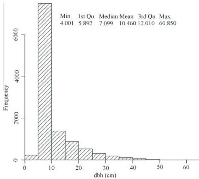
Fig. 2. Histogram and summary statistics of DBH distribution of LiDAR-derived trees in the study area.
