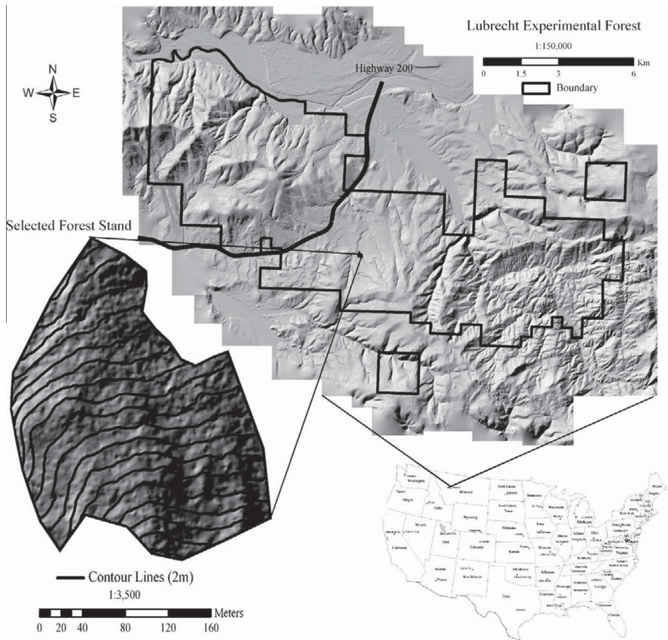
Fig. 1. University of Montana's Lubrecht Experimental Forest boundary and the selected forest stand for the study area.
