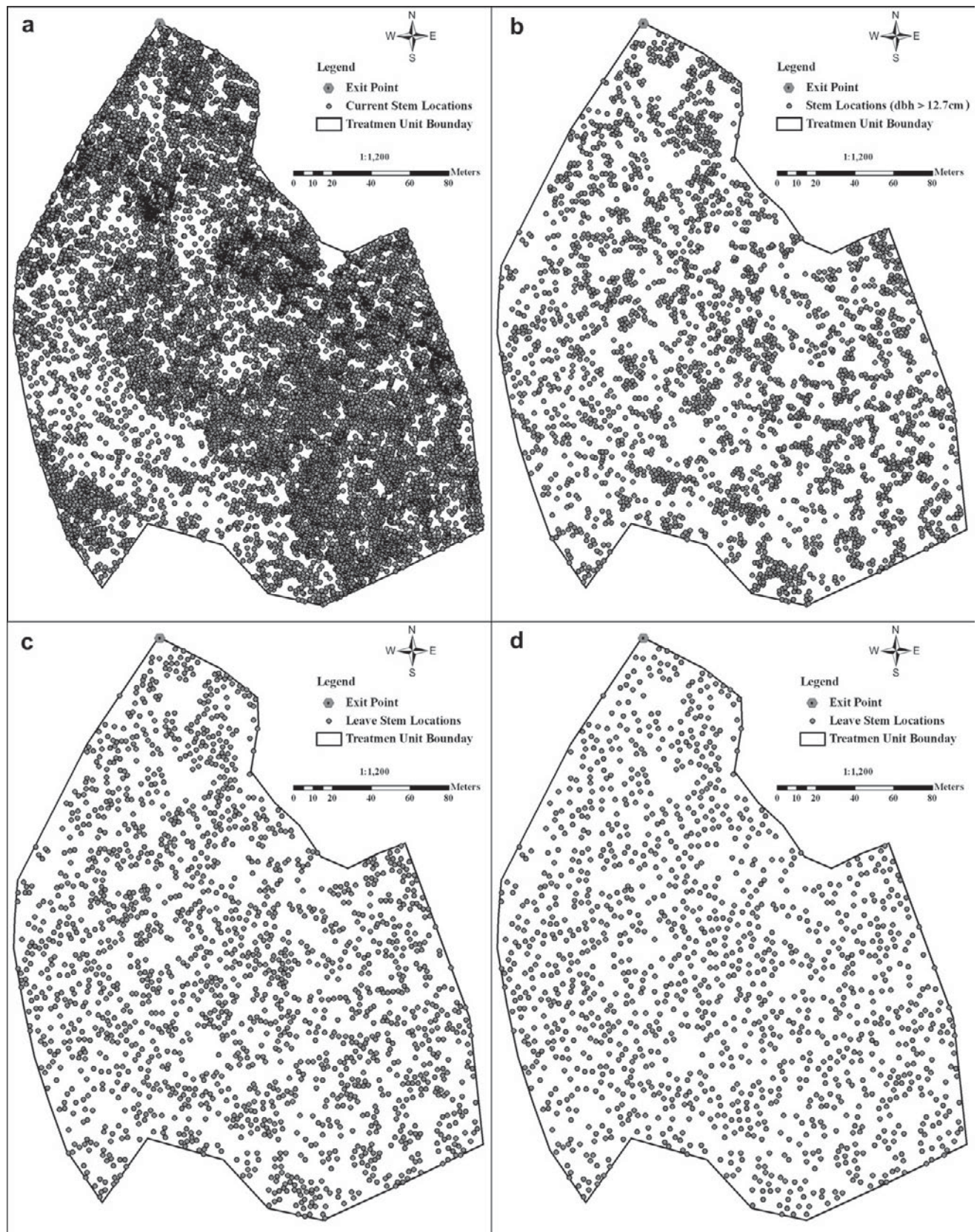
Fig. 5. LiDAR-derived stem map of trees in the study area (a), and location of leave-tree under thinning scenarios I through III, (b) through (d), respectively.
