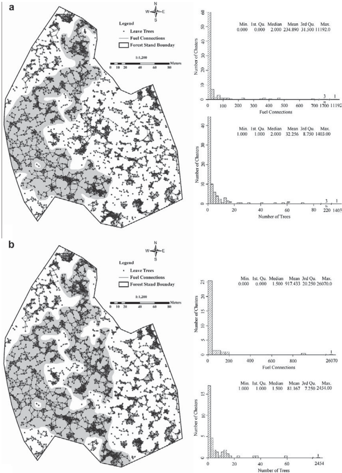
Fig. 7. Location and size of clusters formed by predicted tree-level fuel connections for thinning scenario I under average (a) and severe (b) weather conditions.
