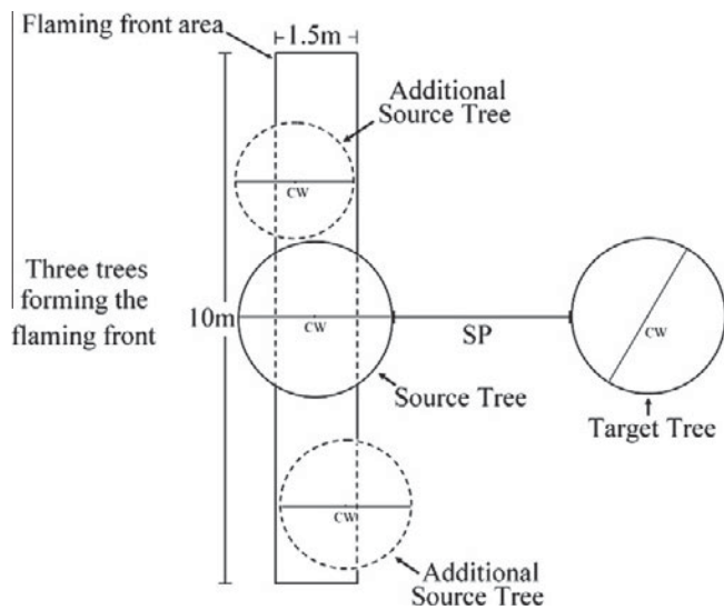
Fig. 6. Schematic of the flaming front area used to estimate crown fire propagation between a source tree and a target tree.
