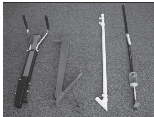
Figure 9. Single-seed planters (from left to right, Hatfield Transplanter, Almaco Hand Jab, Stand 'n Plant, and Seed Stick).
