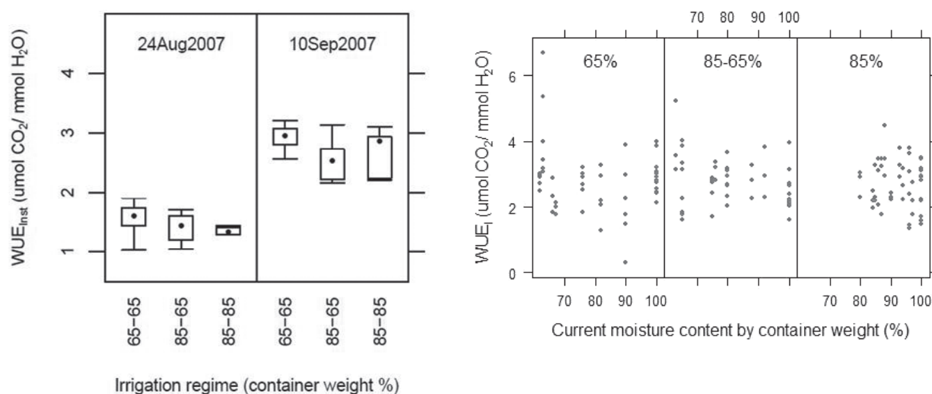
Figure 2. Water use efficiency ( WUE_I ) of Larix occidentalis seedlings following saturation for three irrigation regimes (left) and at varying levels of media moisture content throughout the growing period (right).
