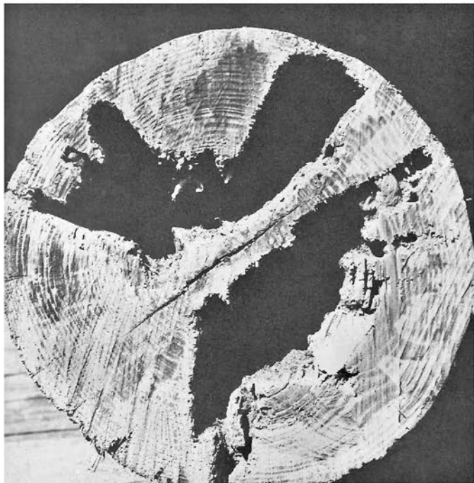
Figure 17A.—Cross section of wedge-shaped hollow.
