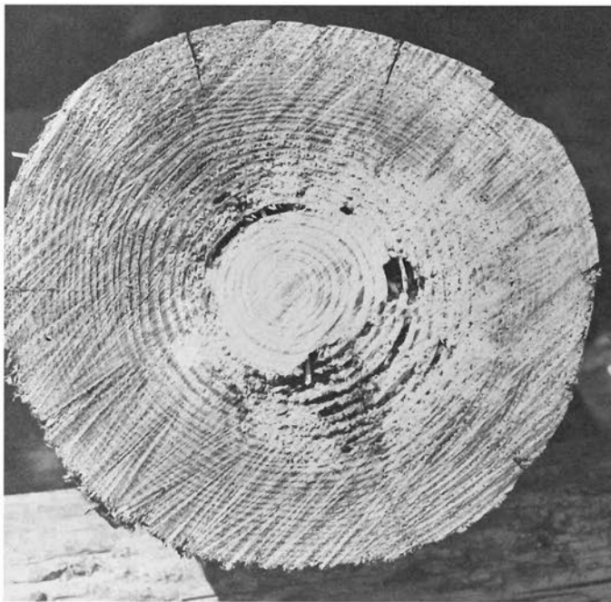
Figure 19.—Early decay (in-between pattern), mostly in spring wood or early wood.
