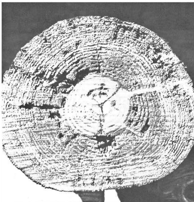
Figure 12A.—Cross section of complete decay.
