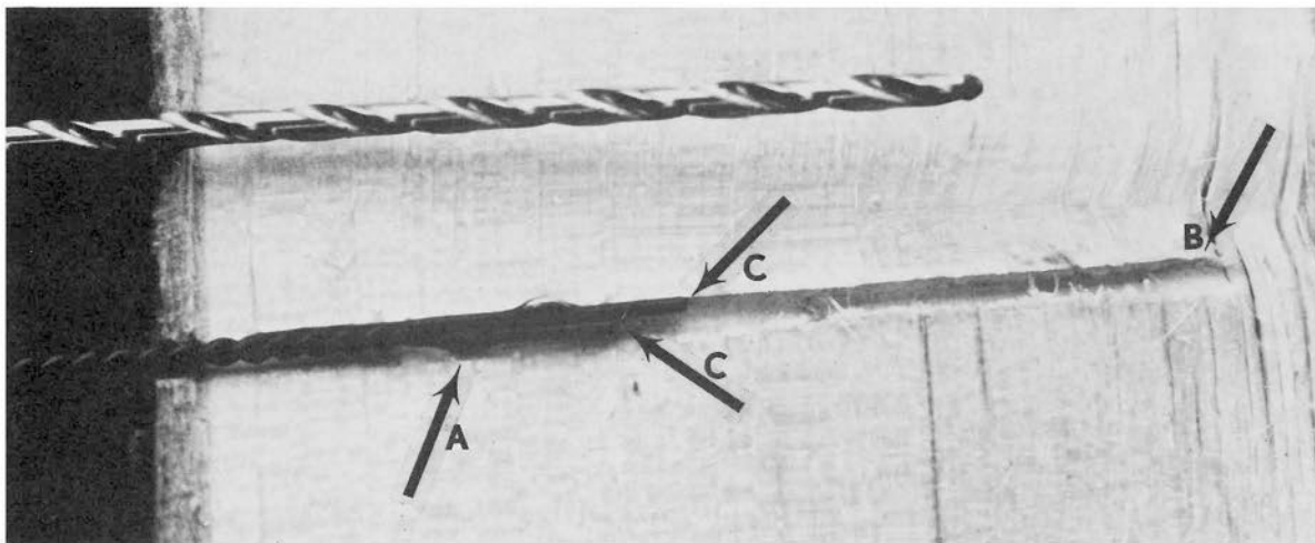
Figure 6.—Closeup of the 3/32-inch diameter drill bit, a hole made by the bit, and the twisted-wire probe in the hole. The arrow (A) points to the back bowed area of the probe tip. The exact depth of a decrease is measured from the surface of the pole to the back bowed area of the tip. Do not record the readings obtained when the probe tip goes to the end of the hole (B). This reading will usually be lower than the others because the open noninsulated tips (C) of the wire make contact with the wood at the end of the hole (B).
