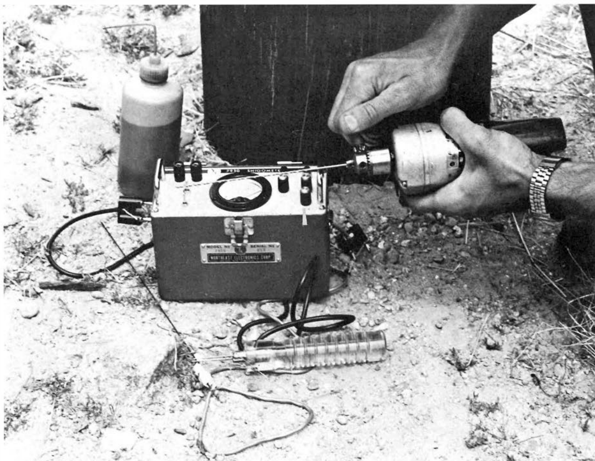
Figure 5A.—Place drill bit firmly in the chuck of drill. If a 12-inch deep hole is desired, make the hole as deep as you can with the 8-inch drill; then complete the job with the 12-inch drill.
