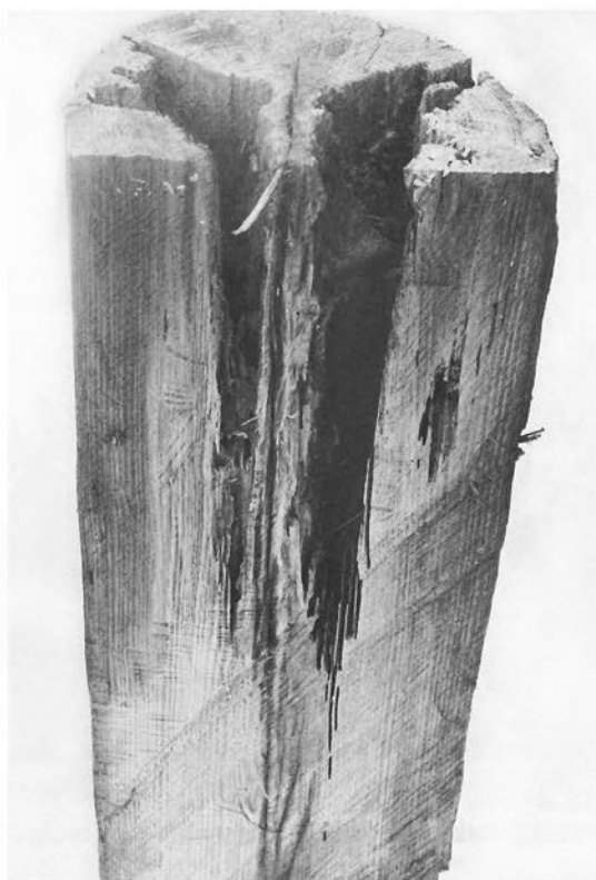
Figure 17B.—Radial section of wedge-shaped hollow.
