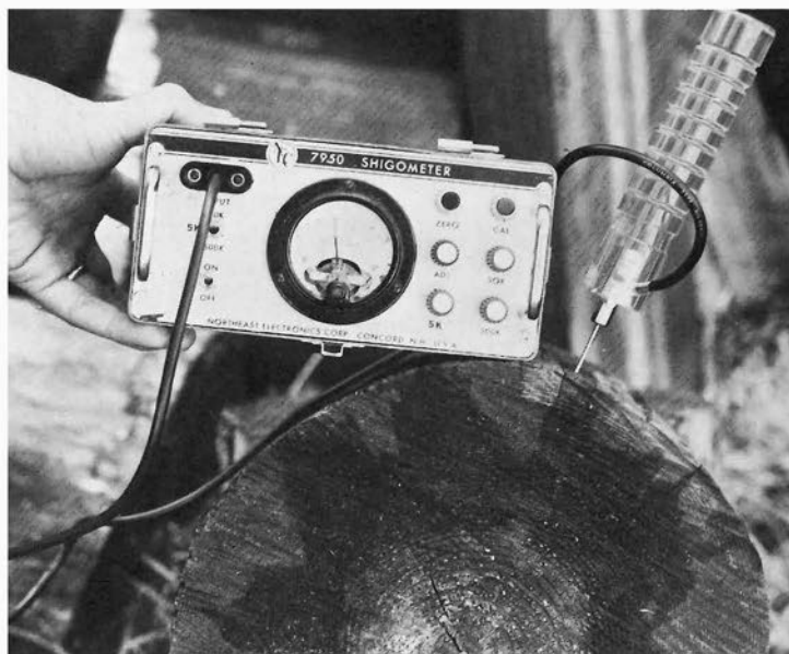
Figure 41.—When it is difficult to push the needle probes into the pole, but very low readings still occur, early deterioration of wood is suspected. When additional probes around such a pole have very high readings, the areas that gave the low readings are all the more suspect. The needle probes shown here are in wood that is beginning to deteriorate; sound zones are also visible on this cross section.
