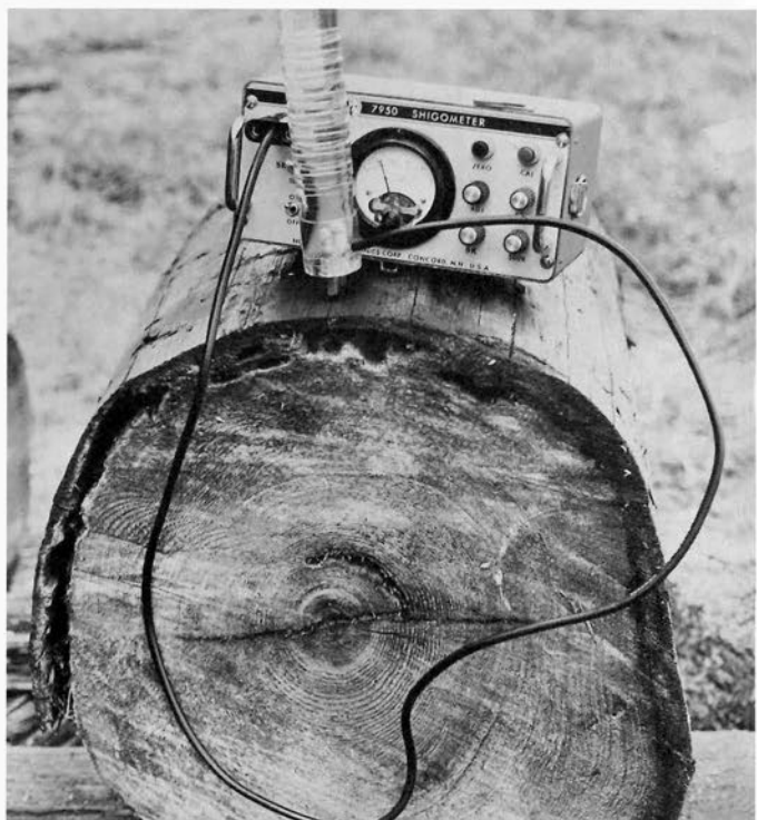
Figure 39.—Easy penetration of the needle probes deep into the pole indicates hollows or decay beneath the surface. Resistance readings below 50 k \Omega also indicate decay.
