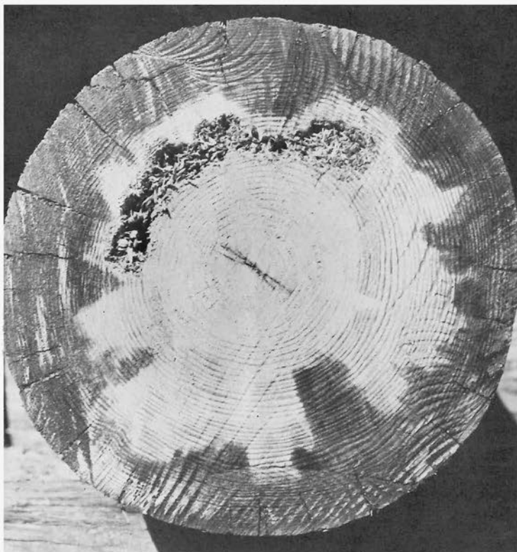
Figure 10A.—Cross section of in-between pattern of decay.
