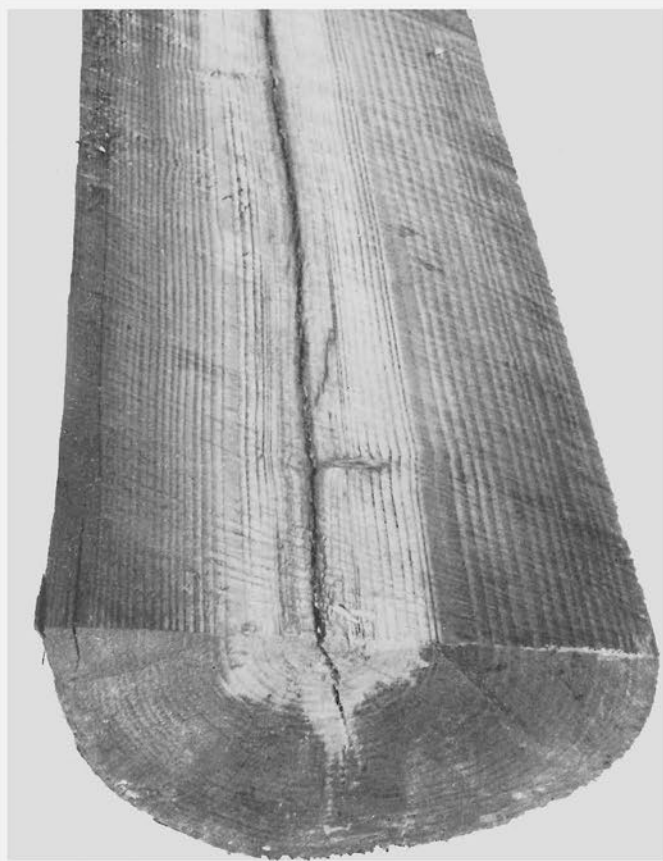
Figure 7B.—Radial section of sound well-treated poles of southern pine.
