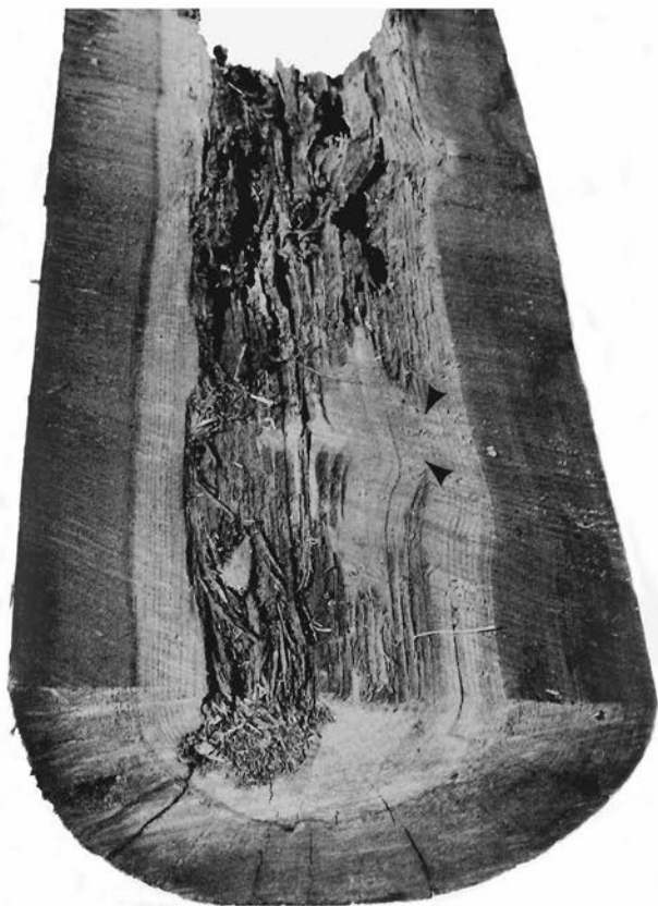
Figure 34.— An increment core at the position marked by the arrow would indicate sound wood. The Shigometer would indicate decay.
