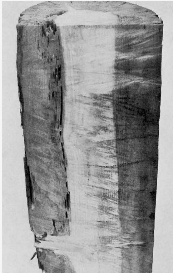
Figure 10B.—Radial section of in-between pattern of decay.
