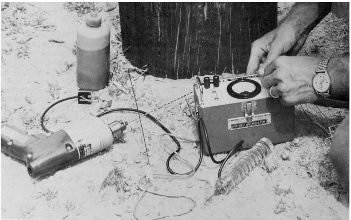
Figure 5B.—Calibrate meter (See Fig. 4). If meter cannot be calibrated, the batteries may be low; put meter on 500 k \Omega scale.
