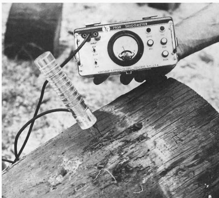
Figure 40.—Needle probes can be used at groundline to detect soft rot. Easy penetration of the wood surface; resistance readings below 50 k \Omega indicates decay.
