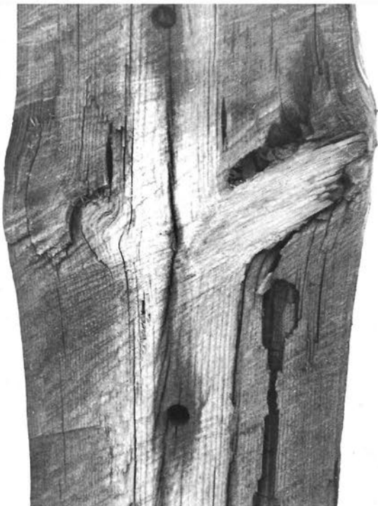
Figure 23.—In-between pattern of decay (brown rot) associated with a large branch stub.
