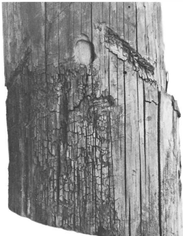
Figure 25.—Wood at groundline that is charred in appearance often indicates soft rot.
