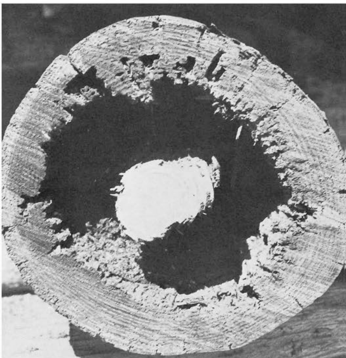
Figure 16A.—Cross section of in-between hollow.
