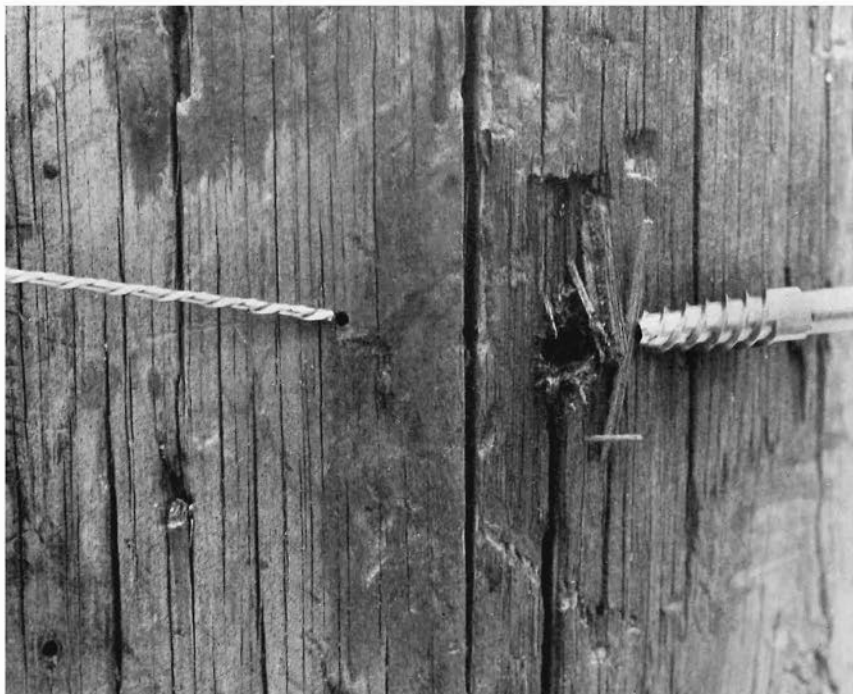
Figure 32.—Holes made by increment borer and drill bit.
