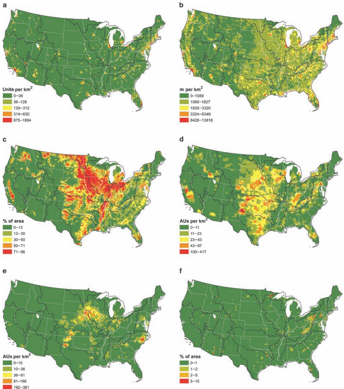
Figure 2. Levels of the stressors: (a) housing density, (b) road density, (c) cultivation, (d) livestock grazing, (e) confined animal feeding, (f) mining land cover, (g) the number of potentially toxic mines, (h) potentially damaging wildfire, (i) atmospheric deposition. Abbreviations: %, percentage; AU, animal units; ha, hectares; kg, kilograms; km 2 , square kilometers; m, meters.
