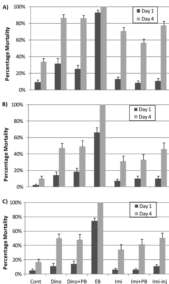
Fig. 1. Cumulative percentage mortality (average + SE) on day 1 and day 4 for A. planipennis beetles provided with Fraxinus sp. foliage in bioassays in June (A), July (B), and August (C) 2007 from untreated control trees (Cont) and trees treated with basal trunk sprays of dinotefuran (Dino) with or without Pentra-Bark (PB), trunk-injected emamectin benzoate (EB), basal trunk sprays of imidacloprid (Imi) with or without Pentra-Bark (PB), or trunk-injected imidacloprid (Imi-inj) ( N = 25 trees per treatment). Main effects of treatment, site, month, and some two-way interactions significantly affected day 1 and day 4 mortality ( P < 0.05 ).
