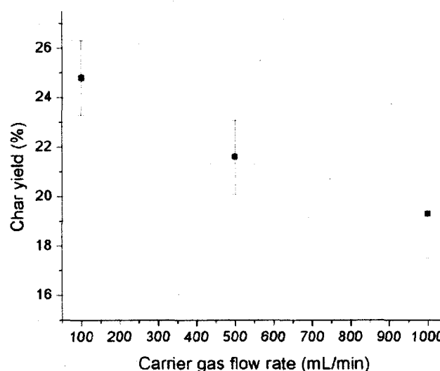
Figure 4. - Effect of purge gas flow rate on the yield of pine chars heated at a final temperature of 500°C for 30 minutes with a heating rate of 30°C/min and nitrogen gas.
