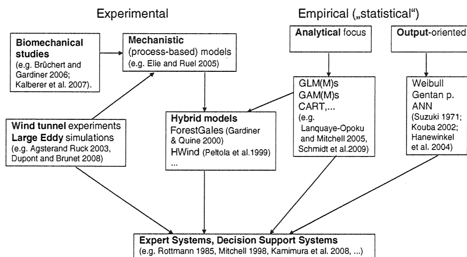
Fig. 2 Overview of methodological approaches for risk assessment and modeling using the example of storm damage. GL(M)Ms generalized linear (mixed) models, GA(M)Ms generalized additive (mixed) models, CART classification and regression trees, ANN artificial neural network
