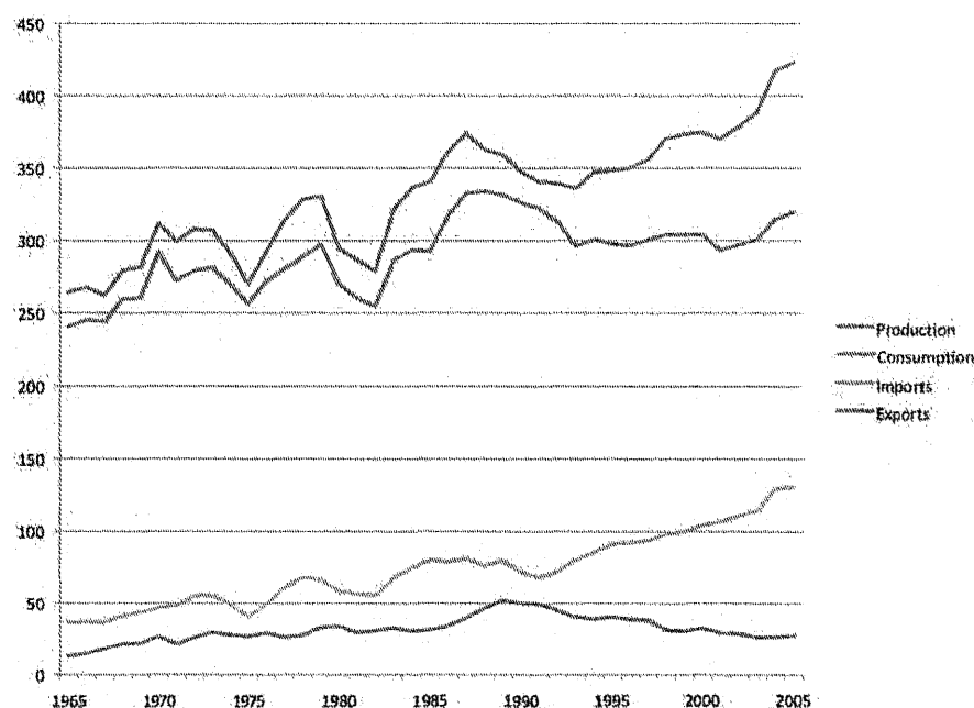
Figure 2-1. Trends in US industrial roundwood, 1965–2005 (million cubic meters). (Source: Howard (2007).)
