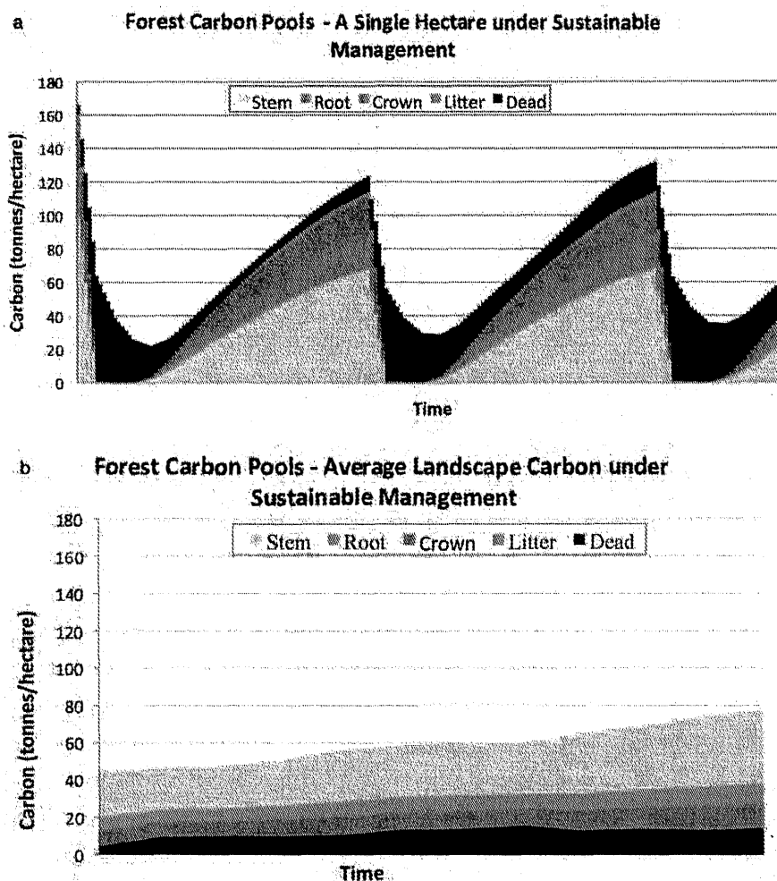
Figure 5-3. Forest carbon under sustainable management, by (a) single hectare and (b) landscape. (Source: Oneil et al. 2011.)
