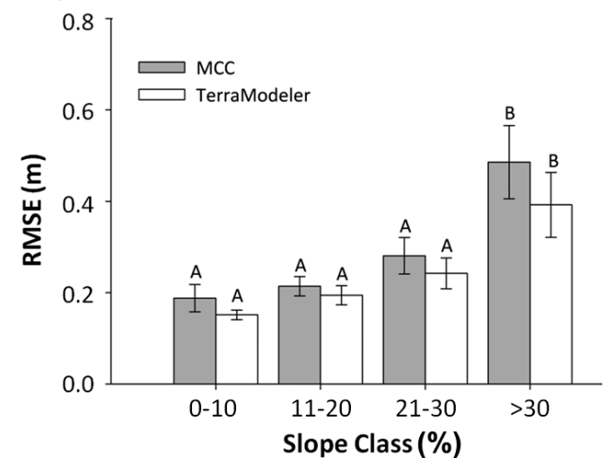
Fig. 5. DEM accuracy within four slope classes, as indicated by the three-way ANOVA. Inset letters represent significant changes in accuracy at the \alpha = 0.05 level.
