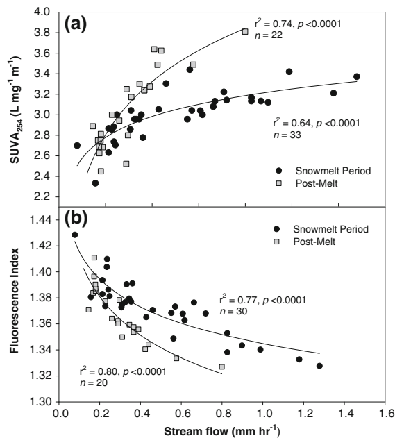
Fig. 5 Regression of DOM compositional indicators a \text{SUVA}_{254} ( \text{L mg}^{-1} \text{m}^{-1} ) and b fluorescence index (FI, unitless) against streamflow ( \text{mm h}^{-1} ) during the active snowmelt period (March 25–April 15, 2009) and post-melt period (April 15–May 13, 2009) at Sleepers River watershed W-9
