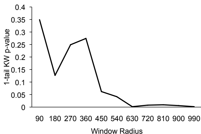
Figure 4. Bivariate scaling plot of 1-tail Kruskal-Wallis p-value for relationship between marten occurrence and landscape-level patch density. The graph indicates highly significant association of marten with low patch density at spatial scales above 450, with highest support at the largest focal extent tested, 990 m.
