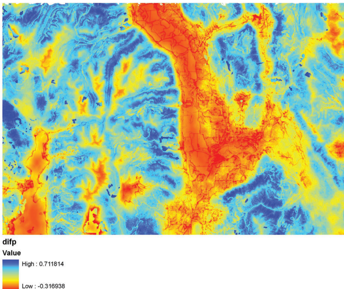
Figure 19. Difference in predicted probability of presence between the optimized scaled model in this paper and a single-scale model from Shirk and others (2011). The areas in blue are predicted to have higher probability of marten occurrence in the scaled model than the unscaled model, while areas in red are predicted to have higher probability of marten occurrence in the unscaled model than the scaled model. The scaled model predicted higher probability of occurrence in high-quality habitat and lower probability of occurrence in low-quality habitat than did the unscaled model.
