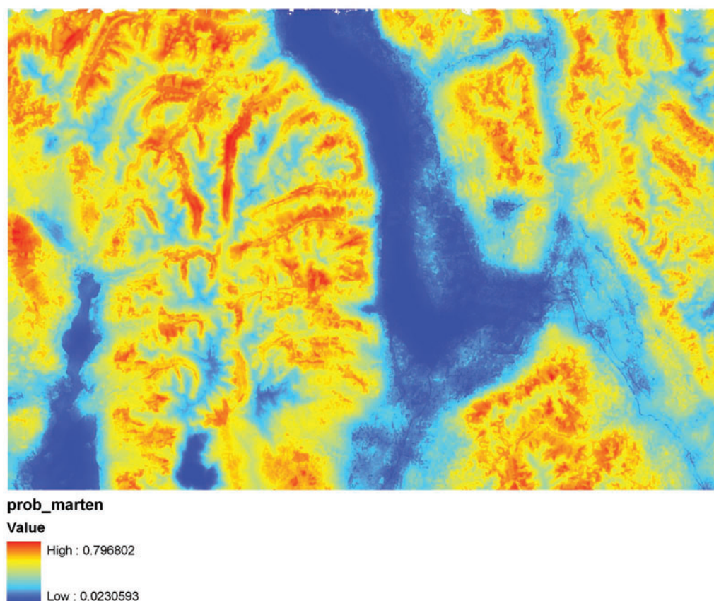
Figure 11. Predicted probability of marten occurrence across the study area as function of the final averaged model.
